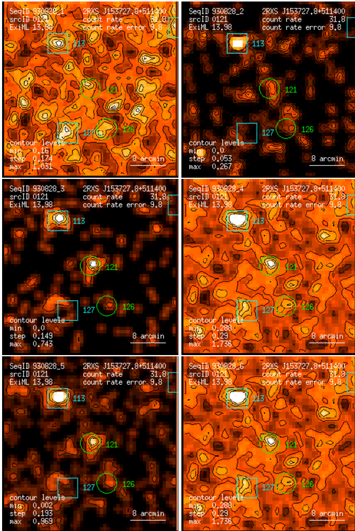
Figure 121: RASS 930828: detection 0121: band rate images, Gaussian filter: (1) PSPC channels 11 – 41, (2) 52 – 90, (3) 91 – 201, (4) 11 – 235, (5) 52 – 201, (6) 11 – 201. Broad band rates in counts/ks. Band rate contour levels in counts/ks/arcmin 2 .
