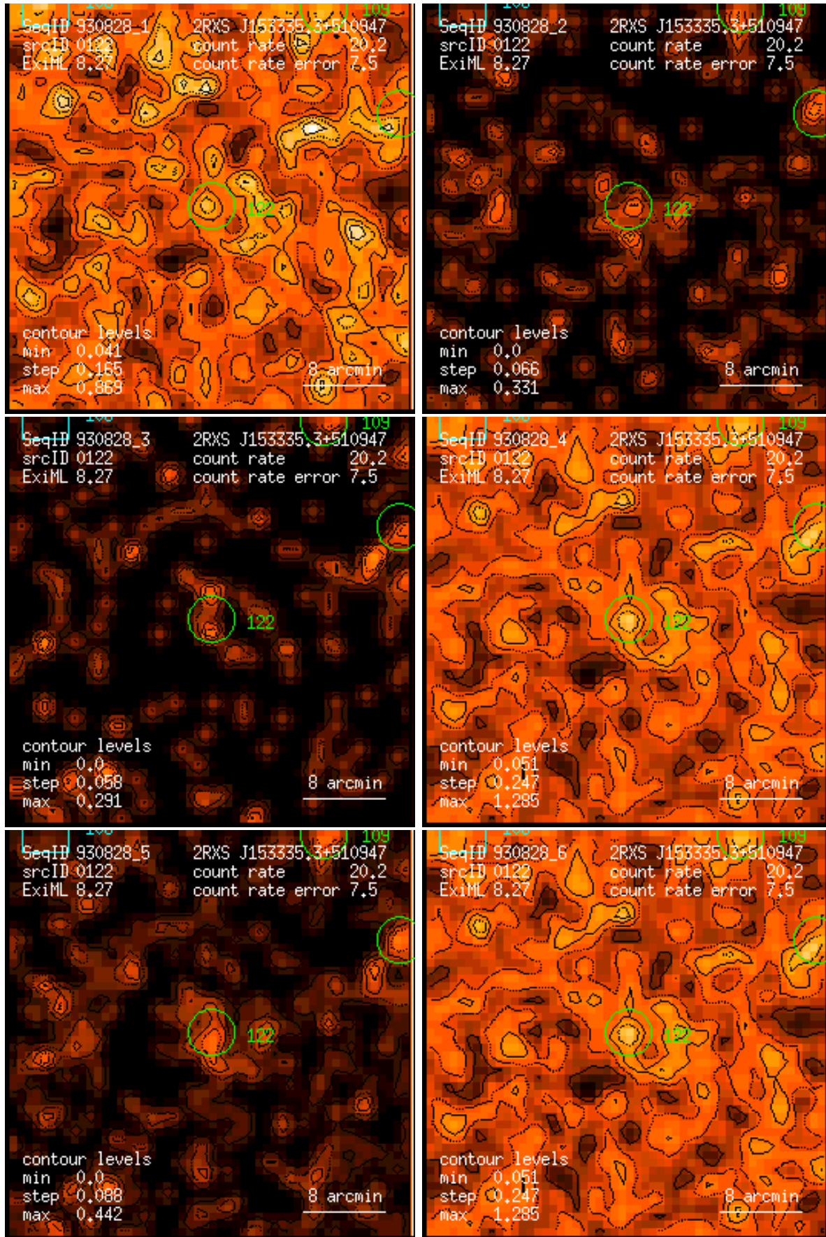
Figure 122: RASS 930828: detection 0122: band rate images, Gaussian filter: (1) PSPC channels 11 – 41, (2) 52 – 90, (3) 91 – 201, (4) 11 – 235, (5) 52 – 201, (6) 11 – 201. Broad band rates in counts/ks. Band rate contour levels in counts/ks/arcmin 2 .
