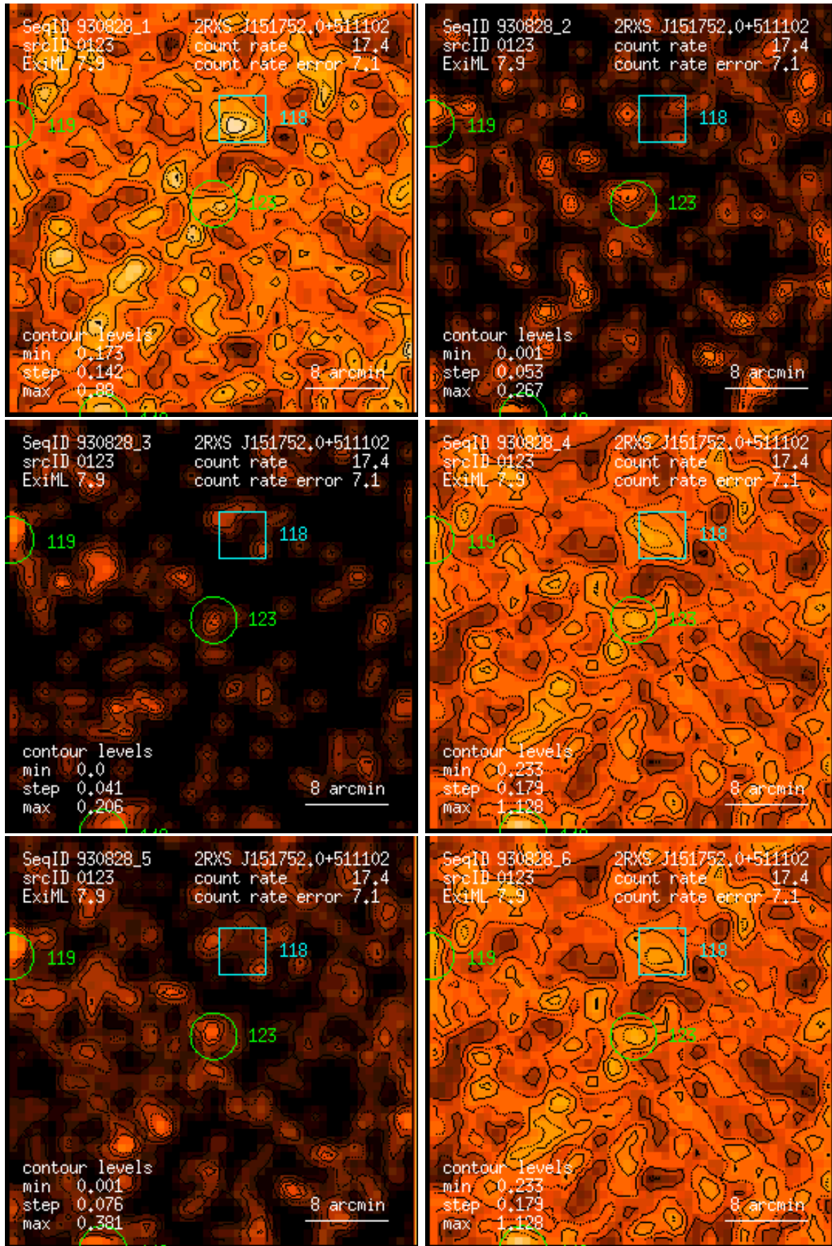
Figure 123: RASS 930828: detection 0123: band rate images, Gaussian filter: (1) PSPC channels 11 – 41, (2) 52 – 90, (3) 91 – 201, (4) 11 – 235, (5) 52 – 201, (6) 11 – 201. Broad band rates in counts/ks. Band rate contour levels in counts/ks/arcmin 2 .
