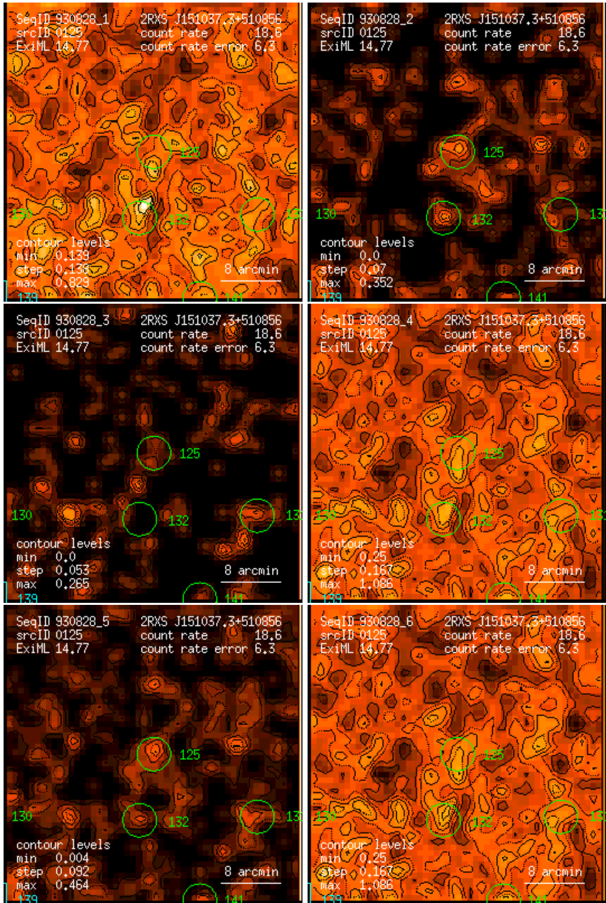
Figure 125: RASS 930828: detection 0125: band rate images, Gaussian filter: (1) PSPC channels 11 – 41, (2) 52 – 90, (3) 91 – 201, (4) 11 – 235, (5) 52 – 201, (6) 11 – 201. Broad band rates in counts/ks. Band rate contour levels in counts/ks/arcmin 2 .
