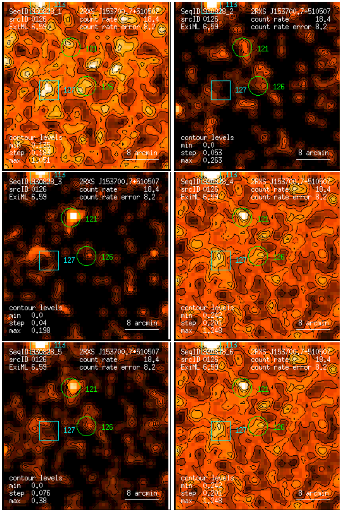
Figure 126: RASS 930828: detection 0126: band rate images, Gaussian filter: (1) PSPC channels 11 – 41, (2) 52 – 90, (3) 91 – 201, (4) 11 – 235, (5) 52 – 201, (6) 11 – 201. Broad band rates in counts/ks. Band rate contour levels in counts/ks/arcmin 2 .
