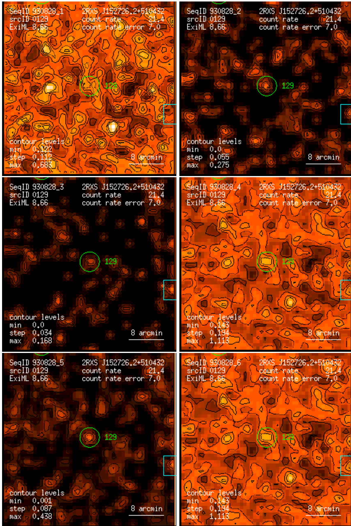
Figure 129: RASS 930828: detection 0129: band rate images, Gaussian filter: (1) PSPC channels 11 – 41, (2) 52 – 90, (3) 91 – 201, (4) 11 – 235, (5) 52 – 201, (6) 11 – 201. Broad band rates in counts/ks. Band rate contour levels in counts/ks/arcmin 2 .
