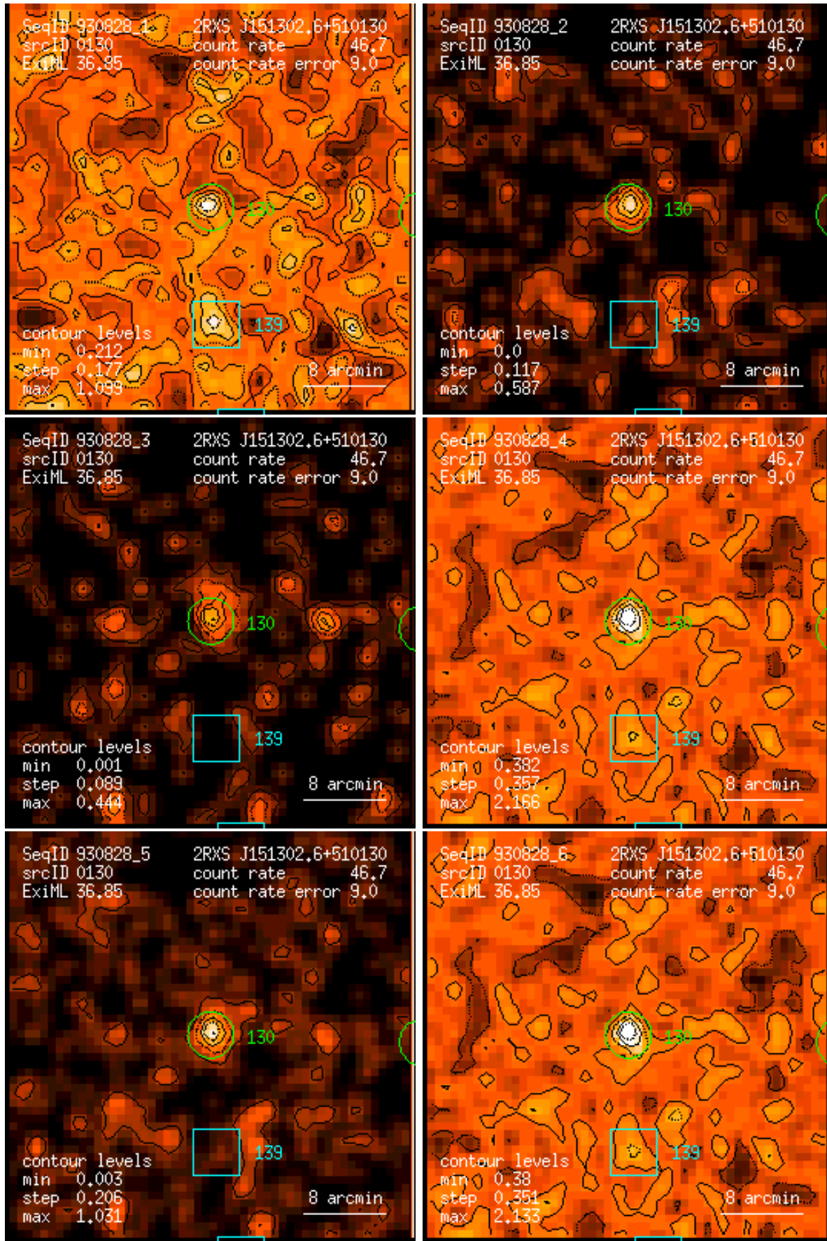
Figure 130: RASS 930828: detection 0130: band rate images, Gaussian filter: (1) PSPC channels 11 – 41, (2) 52 – 90, (3) 91 – 201, (4) 11 – 235, (5) 52 – 201, (6) 11 – 201. Broad band rates in counts/ks. Band rate contour levels in counts/ks/arcmin 2 .
