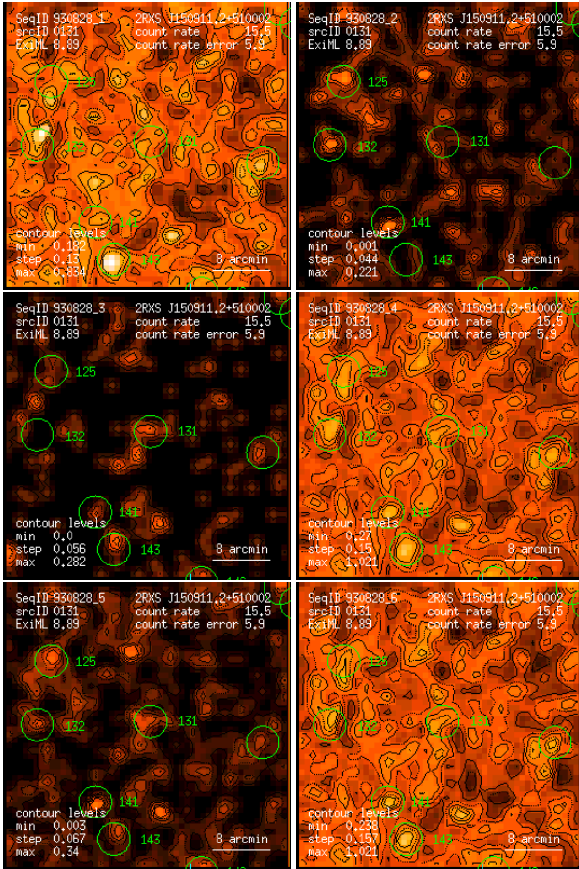
Figure 131: RASS 930828: detection 0131: band rate images, Gaussian filter: (1) PSPC channels 11 – 41, (2) 52 – 90, (3) 91 – 201, (4) 11 – 235, (5) 52 – 201, (6) 11 – 201. Broad band rates in counts/ks. Band rate contour levels in counts/ks/arcmin 2 .
