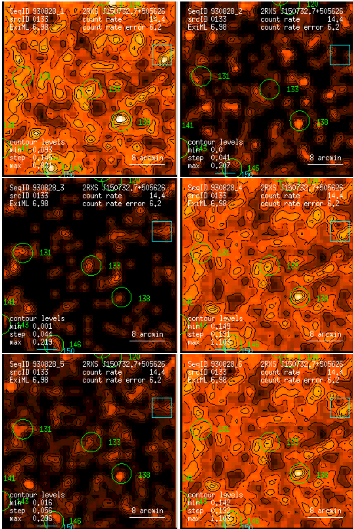
Figure 133: RASS 930828: detection 0133: band rate images, Gaussian filter: (1) PSPC channels 11 – 41, (2) 52 – 90, (3) 91 – 201, (4) 11 – 235, (5) 52 – 201, (6) 11 – 201. Broad band rates in counts/ks. Band rate contour levels in counts/ks/arcmin 2 .
