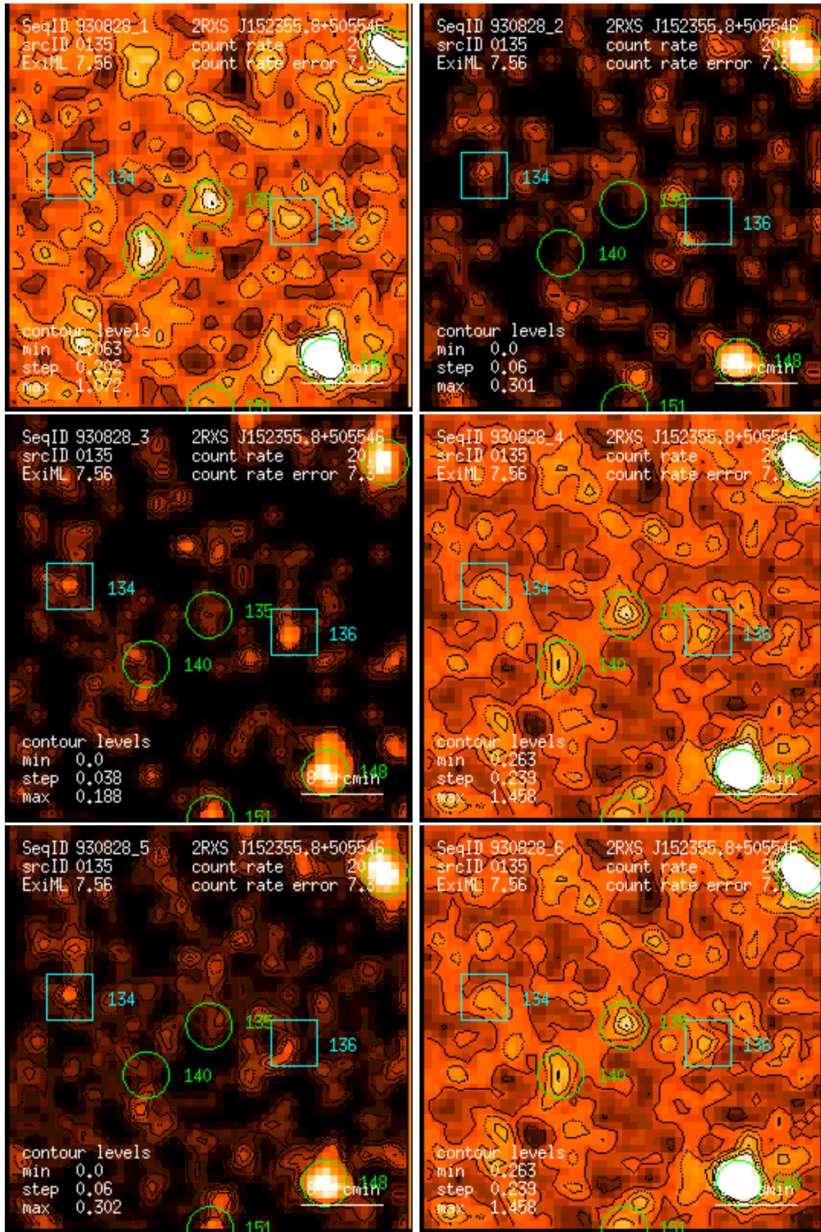
Figure 135: RASS 930828: detection 0135: band rate images, Gaussian filter: (1) PSPC channels 11 – 41, (2) 52 – 90, (3) 91 – 201, (4) 11 – 235, (5) 52 – 201, (6) 11 – 201. Broad band rates in counts/ks. Band rate contour levels in counts/ks/arcmin 2 .
