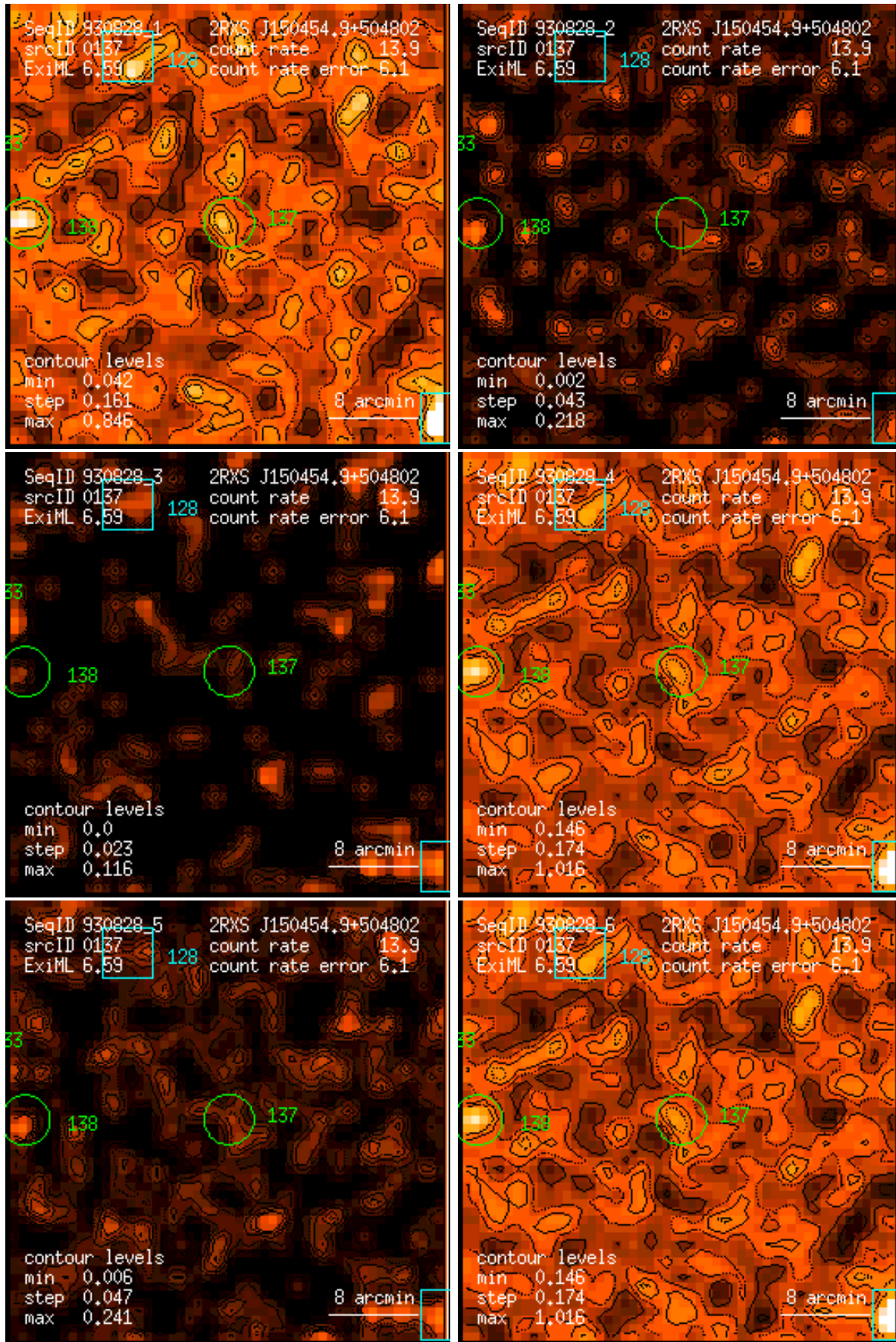
Figure 137: RASS 930828: detection 0137: band rate images, Gaussian filter: (1) PSPC channels 11 – 41, (2) 52 – 90, (3) 91 – 201, (4) 11 – 235, (5) 52 – 201, (6) 11 – 201. Broad band rates in counts/ks. Band rate contour levels in counts/ks/arcmin 2 .
