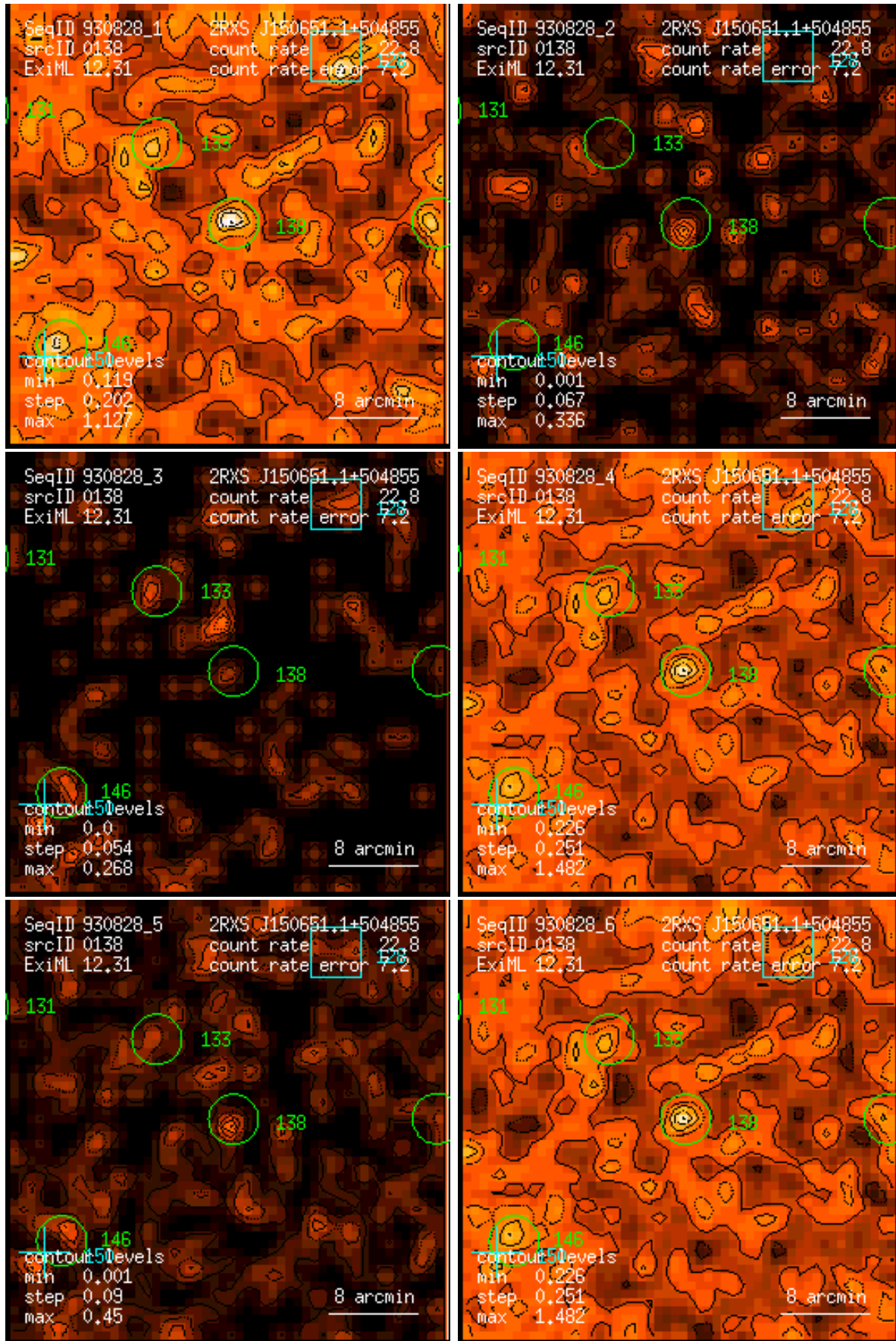
Figure 138: RASS 930828: detection 0138: band rate images, Gaussian filter: (1) PSPC channels 11 – 41, (2) 52 – 90, (3) 91 – 201, (4) 11 – 235, (5) 52 – 201, (6) 11 – 201. Broad band rates in counts/ks. Band rate contour levels in counts/ks/arcmin 2 .
