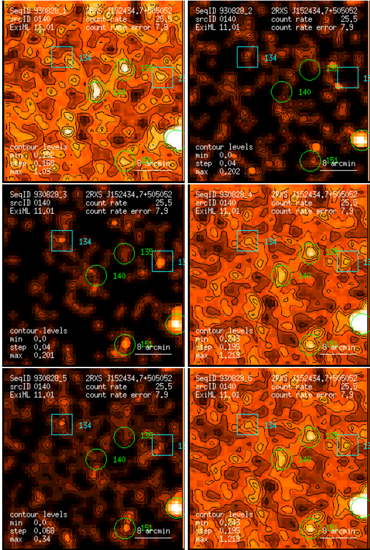
Figure 140: RASS 930828: detection 0140: band rate images, Gaussian filter: (1) PSPC channels 11 – 41, (2) 52 – 90, (3) 91 – 201, (4) 11 – 235, (5) 52 – 201, (6) 11 – 201. Broad band rates in counts/ks. Band rate contour levels in counts/ks/arcmin 2 .
