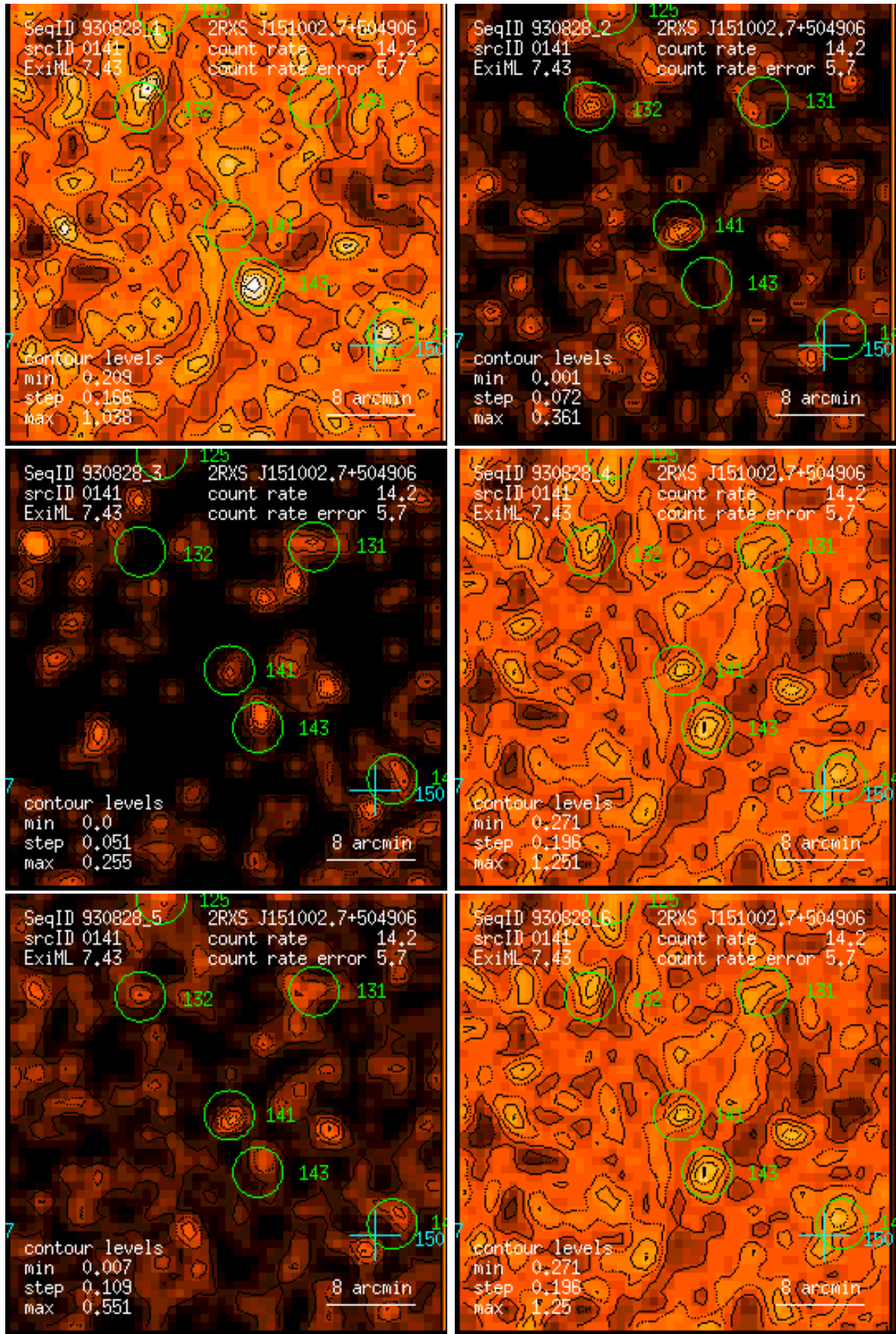
Figure 141: RASS 930828: detection 0141: band rate images, Gaussian filter: (1) PSPC channels 11 – 41, (2) 52 – 90, (3) 91 – 201, (4) 11 – 235, (5) 52 – 201, (6) 11 – 201. Broad band rates in counts/ks. Band rate contour levels in counts/ks/arcmin 2 .
