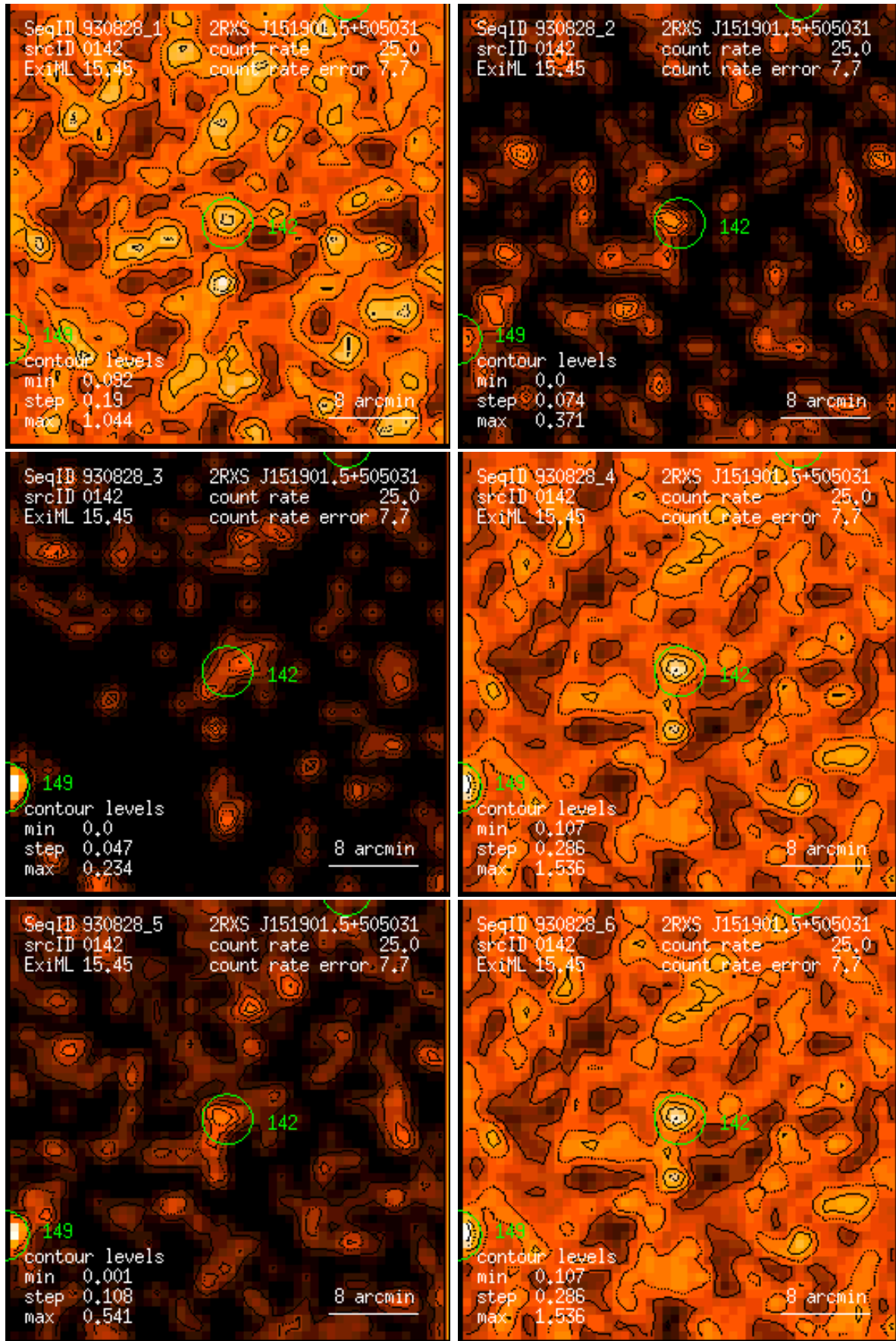
Figure 142: RASS 930828: detection 0142: band rate images, Gaussian filter: (1) PSPC channels 11 – 41, (2) 52 – 90, (3) 91 – 201, (4) 11 – 235, (5) 52 – 201, (6) 11 – 201. Broad band rates in counts/ks. Band rate contour levels in counts/ks/arcmin 2 .
