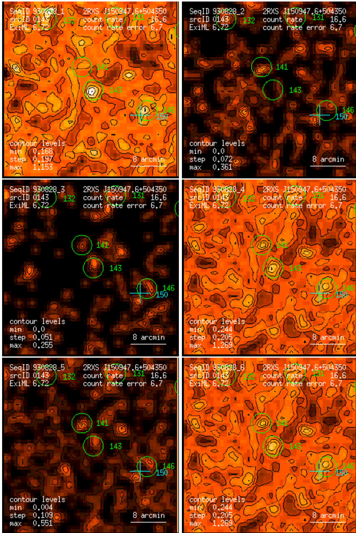
Figure 143: RASS 930828: detection 0143: band rate images, Gaussian filter: (1) PSPC channels 11 – 41, (2) 52 – 90, (3) 91 – 201, (4) 11 – 235, (5) 52 – 201, (6) 11 – 201. Broad band rates in counts/ks. Band rate contour levels in counts/ks/arcmin 2 .
