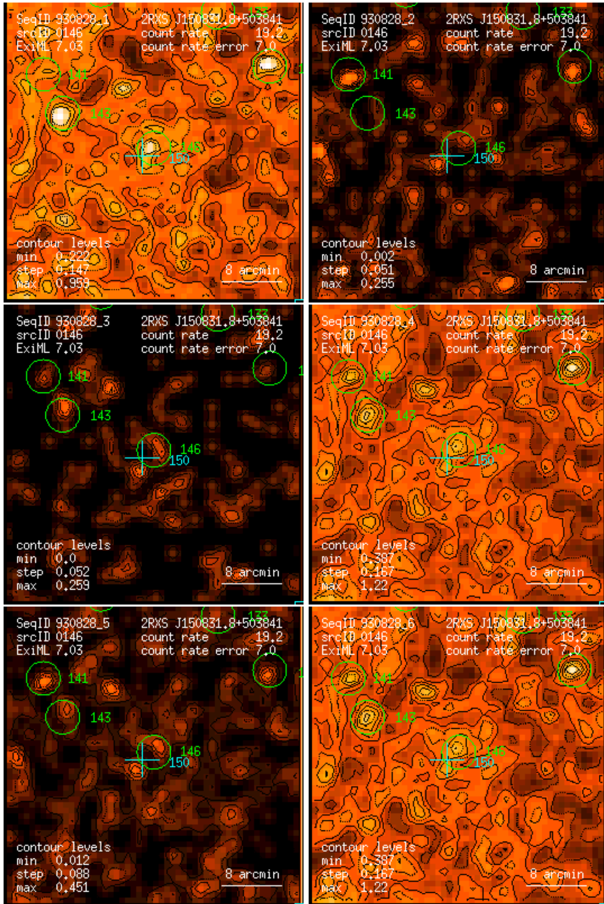
Figure 146: RASS 930828: detection 0146: band rate images, Gaussian filter: (1) PSPC channels 11 – 41, (2) 52 – 90, (3) 91 – 201, (4) 11 – 235, (5) 52 – 201, (6) 11 – 201. Broad band rates in counts/ks. Band rate contour levels in counts/ks/arcmin 2 .
