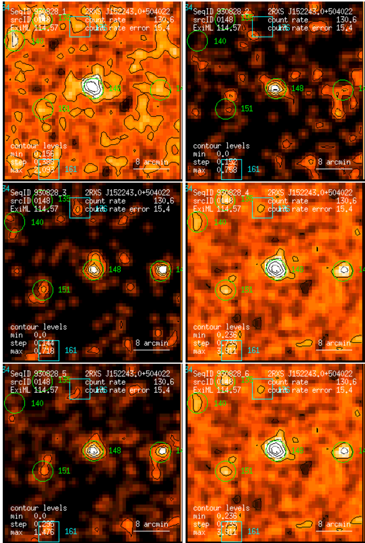
Figure 148: RASS 930828: detection 0148: band rate images, Gaussian filter: (1) PSPC channels 11 – 41, (2) 52 – 90, (3) 91 – 201, (4) 11 – 235, (5) 52 – 201, (6) 11 – 201. Broad band rates in counts/ks. Band rate contour levels in counts/ks/arcmin 2 .
