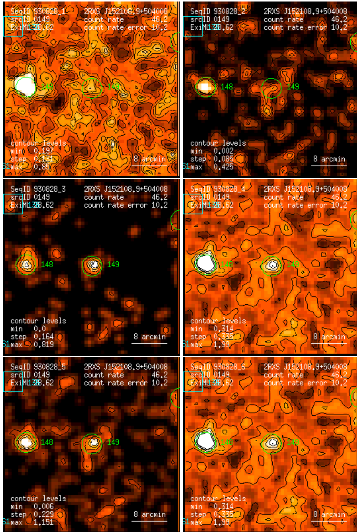
Figure 149: RASS 930828: detection 0149: band rate images, Gaussian filter: (1) PSPC channels 11 – 41, (2) 52 – 90, (3) 91 – 201, (4) 11 – 235, (5) 52 – 201, (6) 11 – 201. Broad band rates in counts/ks. Band rate contour levels in counts/ks/arcmin 2 .
