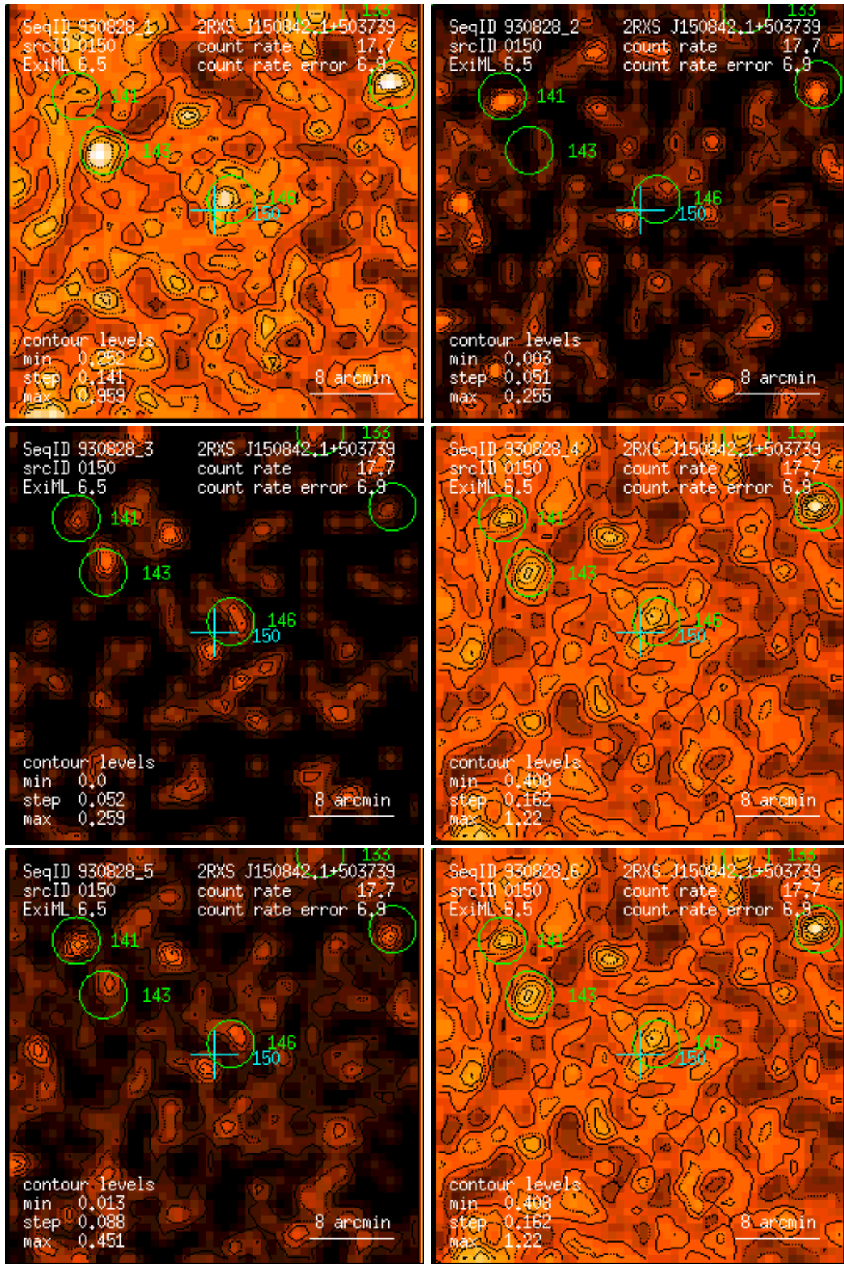
Figure 150: RASS 930828: detection 0150: band rate images, Gaussian filter: (1) PSPC channels 11 – 41, (2) 52 – 90, (3) 91 – 201, (4) 11 – 235, (5) 52 – 201, (6) 11 – 201. Broad band rates in counts/ks. Band rate contour levels in counts/ks/arcmin 2 .
