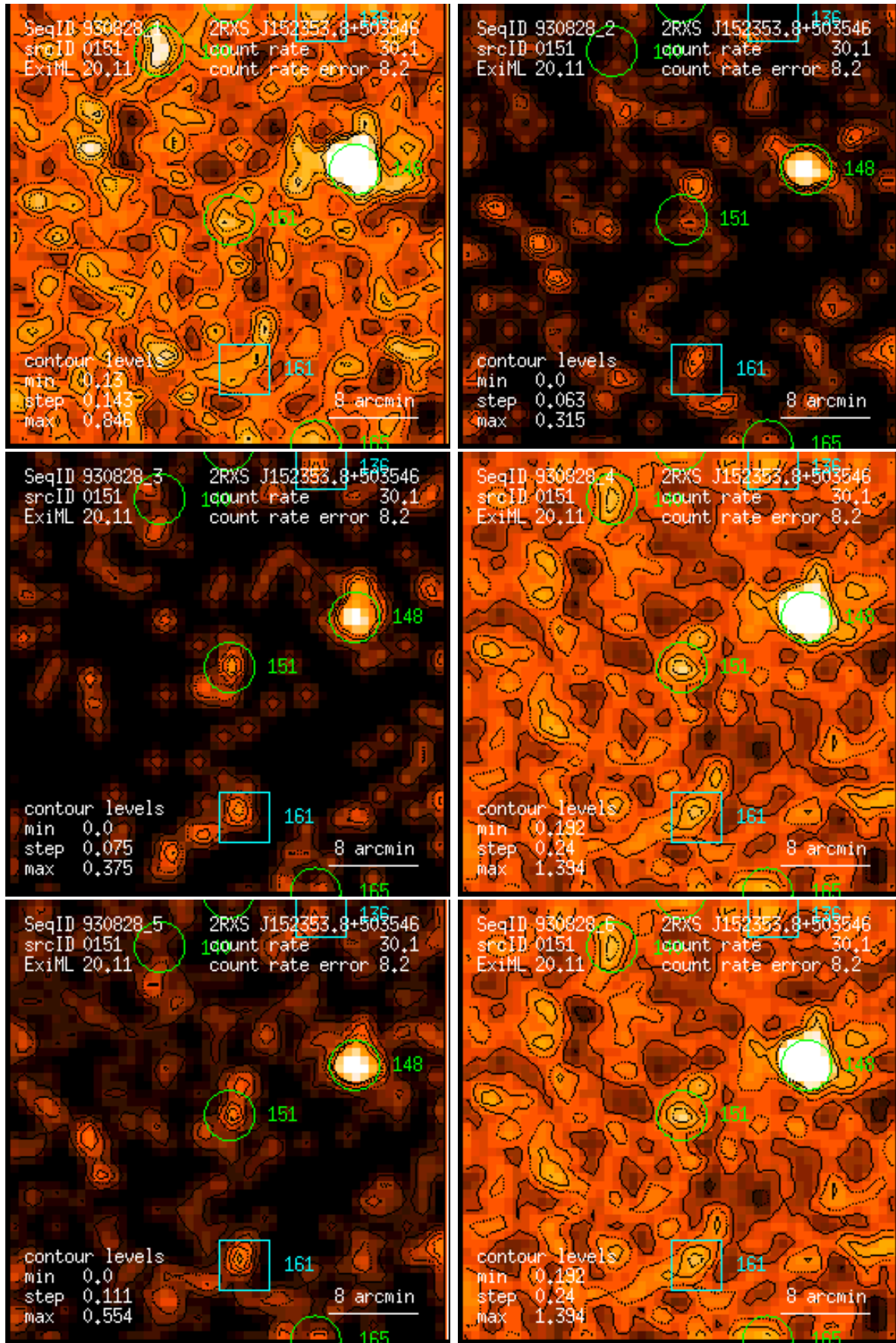
Figure 151: RASS 930828: detection 0151: band rate images, Gaussian filter: (1) PSPC channels 11 – 41, (2) 52 – 90, (3) 91 – 201, (4) 11 – 235, (5) 52 – 201, (6) 11 – 201. Broad band rates in counts/ks. Band rate contour levels in counts/ks/arcmin 2 .
