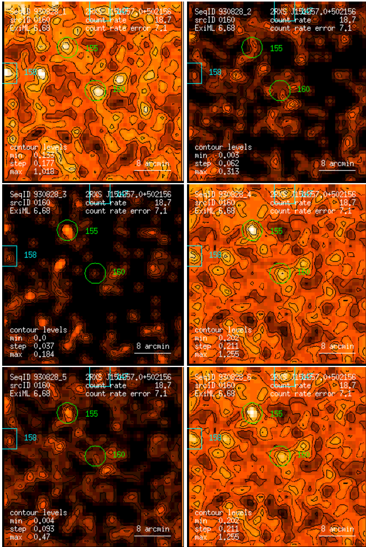
Figure 160: RASS 930828: detection 0160: band rate images, Gaussian filter: (1) PSPC channels 11 – 41, (2) 52 – 90, (3) 91 – 201, (4) 11 – 235, (5) 52 – 201, (6) 11 – 201. Broad band rates in counts/ks. Band rate contour levels in counts/ks/arcmin 2 .
