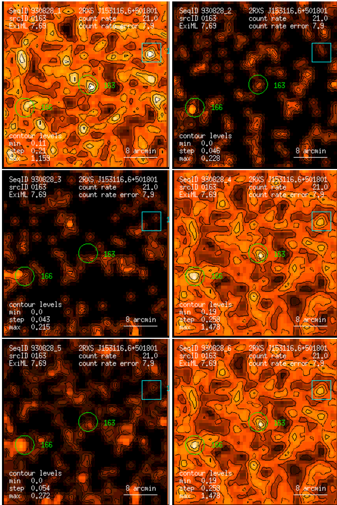
Figure 163: RASS 930828: detection 0163: band rate images, Gaussian filter: (1) PSPC channels 11 – 41, (2) 52 – 90, (3) 91 – 201, (4) 11 – 235, (5) 52 – 201, (6) 11 – 201. Broad band rates in counts/ks. Band rate contour levels in counts/ks/arcmin 2 .
