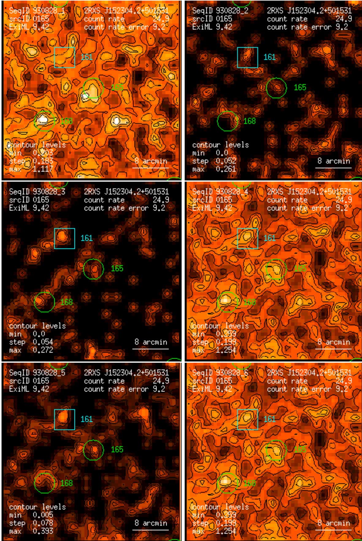
Figure 165: RASS 930828: detection 0165: band rate images, Gaussian filter: (1) PSPC channels 11 – 41, (2) 52 – 90, (3) 91 – 201, (4) 11 – 235, (5) 52 – 201, (6) 11 – 201. Broad band rates in counts/ks. Band rate contour levels in counts/ks/arcmin 2 .
