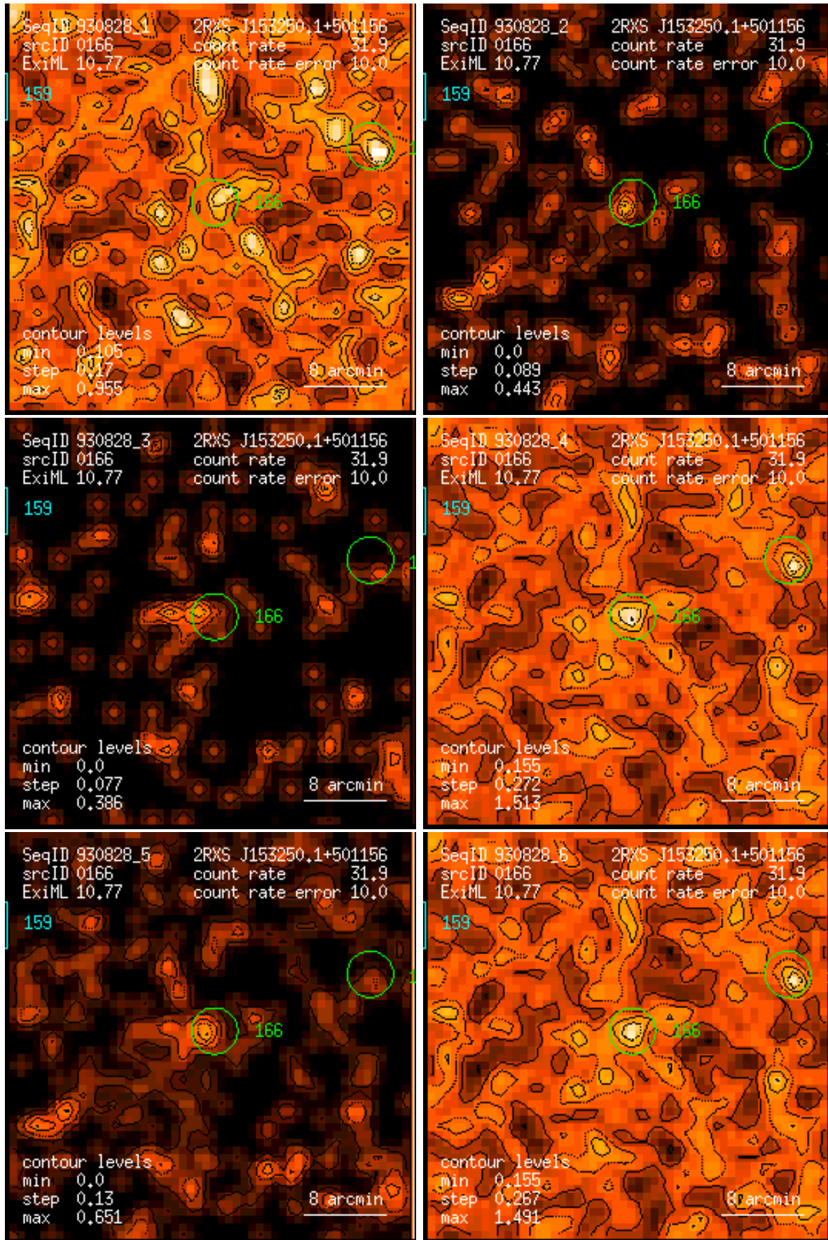
Figure 166: RASS 930828: detection 0166: band rate images, Gaussian filter: (1) PSPC channels 11 – 41, (2) 52 – 90, (3) 91 – 201, (4) 11 – 235, (5) 52 – 201, (6) 11 – 201. Broad band rates in counts/ks. Band rate contour levels in counts/ks/arcmin 2 .
