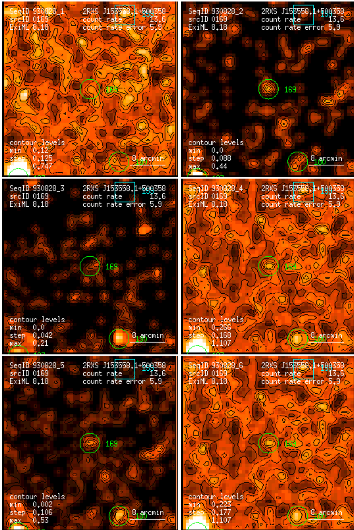
Figure 169: RASS 930828: detection 0169: band rate images, Gaussian filter: (1) PSPC channels 11 – 41, (2) 52 – 90, (3) 91 – 201, (4) 11 – 235, (5) 52 – 201, (6) 11 – 201. Broad band rates in counts/ks. Band rate contour levels in counts/ks/arcmin 2 .
