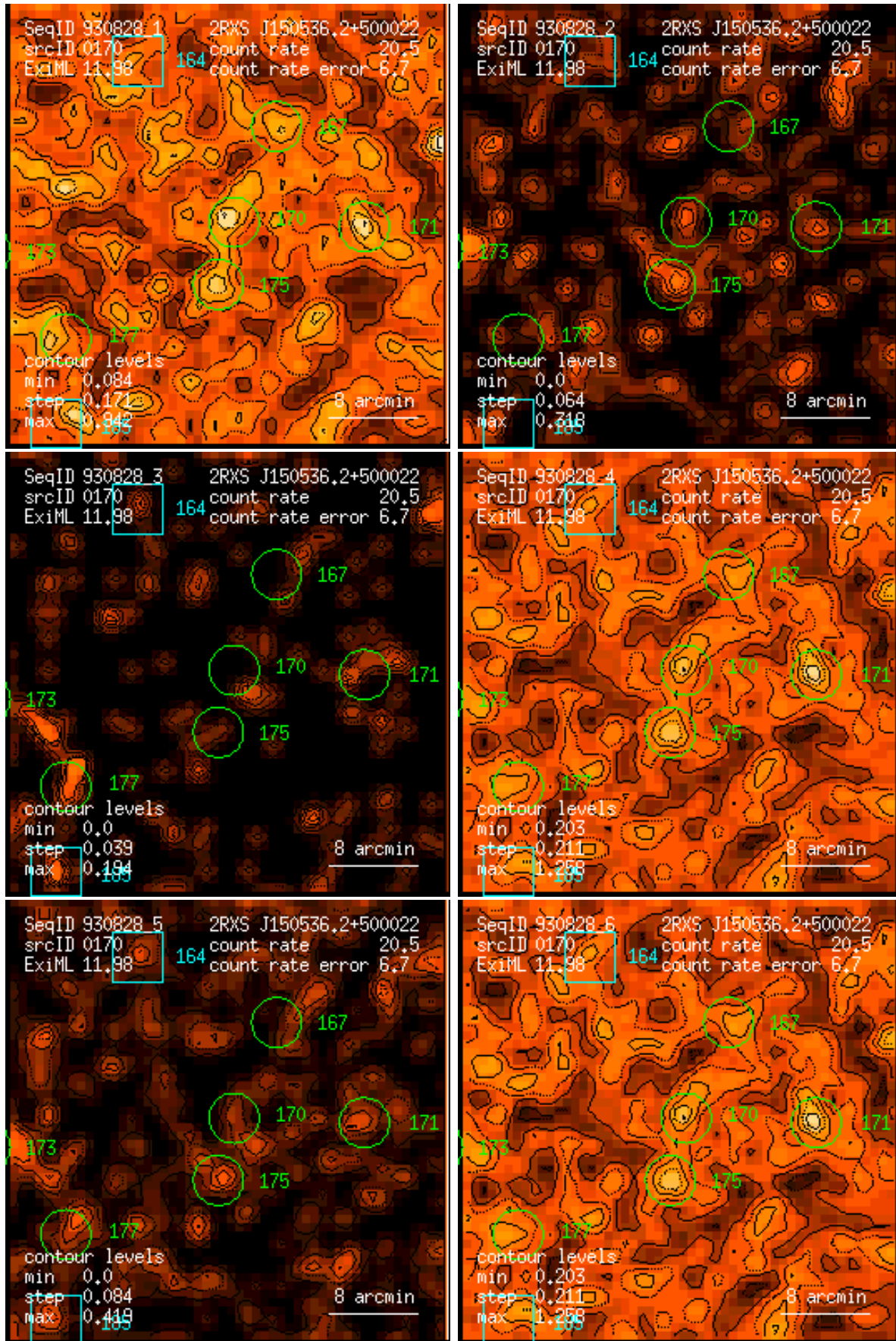
Figure 170: RASS 930828: detection 0170: band rate images, Gaussian filter: (1) PSPC channels 11 – 41, (2) 52 – 90, (3) 91 – 201, (4) 11 – 235, (5) 52 – 201, (6) 11 – 201. Broad band rates in counts/ks. Band rate contour levels in counts/ks/arcmin 2 .
