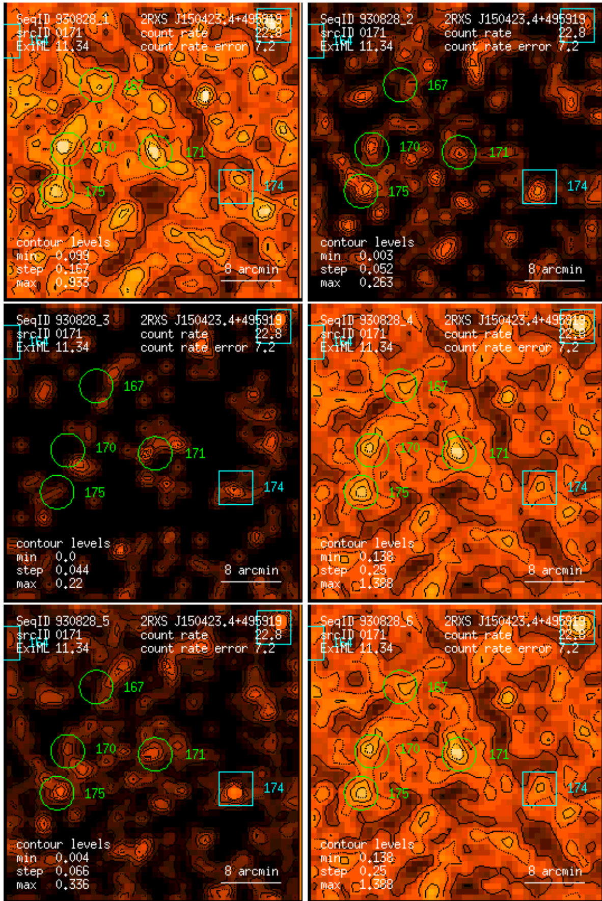
Figure 171: RASS 930828: detection 0171: band rate images, Gaussian filter: (1) PSPC channels 11 – 41, (2) 52 – 90, (3) 91 – 201, (4) 11 – 235, (5) 52 – 201, (6) 11 – 201. Broad band rates in counts/ks. Band rate contour levels in counts/ks/arcmin 2 .
