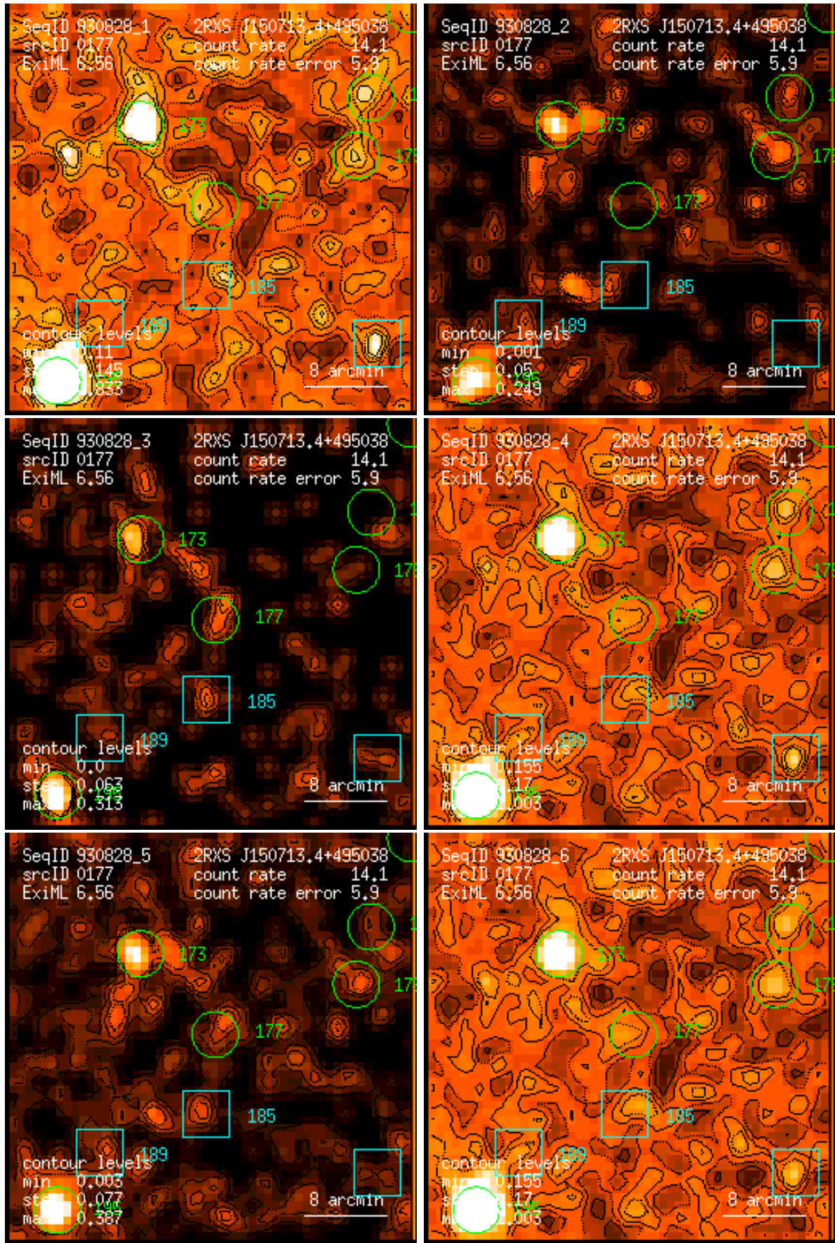
Figure 177: RASS 930828: detection 0177: band rate images, Gaussian filter: (1) PSPC channels 11 – 41, (2) 52 – 90, (3) 91 – 201, (4) 11 – 235, (5) 52 – 201, (6) 11 – 201. Broad band rates in counts/ks. Band rate contour levels in counts/ks/arcmin 2 .
