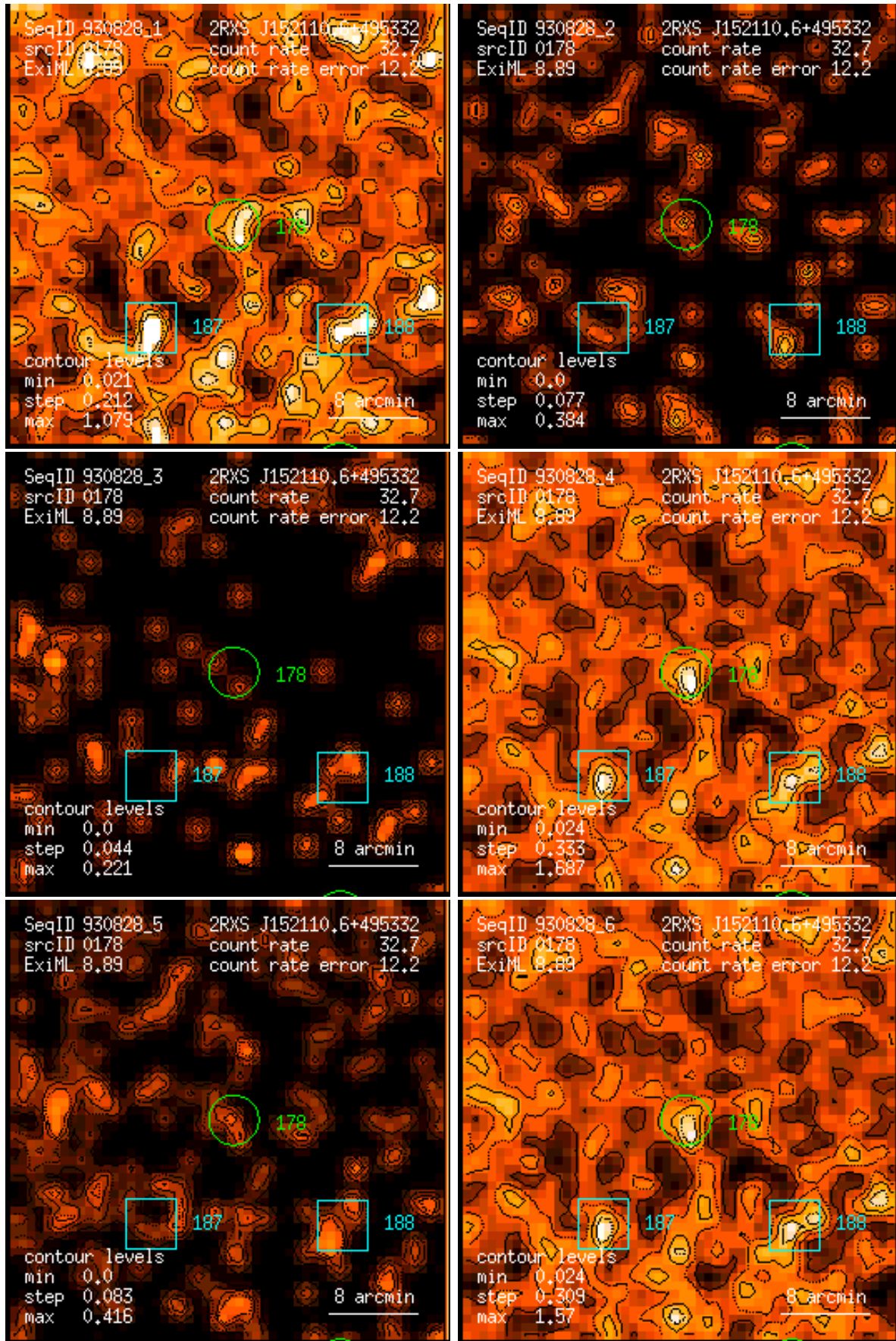
Figure 178: RASS 930828: detection 0178: band rate images, Gaussian filter: (1) PSPC channels 11 – 41, (2) 52 – 90, (3) 91 – 201, (4) 11 – 235, (5) 52 – 201, (6) 11 – 201. Broad band rates in counts/ks. Band rate contour levels in counts/ks/arcmin 2 .
