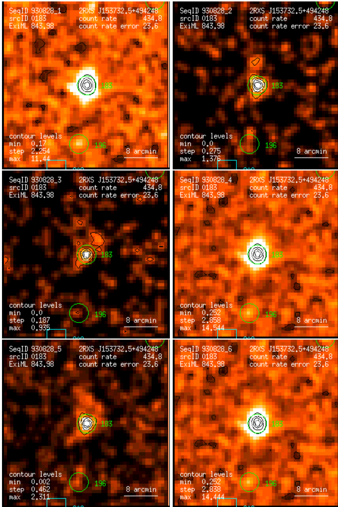
Figure 183: RASS 930828: detection 0183: band rate images, Gaussian filter: (1) PSPC channels 11 – 41, (2) 52 – 90, (3) 91 – 201, (4) 11 – 235, (5) 52 – 201, (6) 11 – 201. Broad band rates in counts/ks. Band rate contour levels in counts/ks/arcmin 2 .
