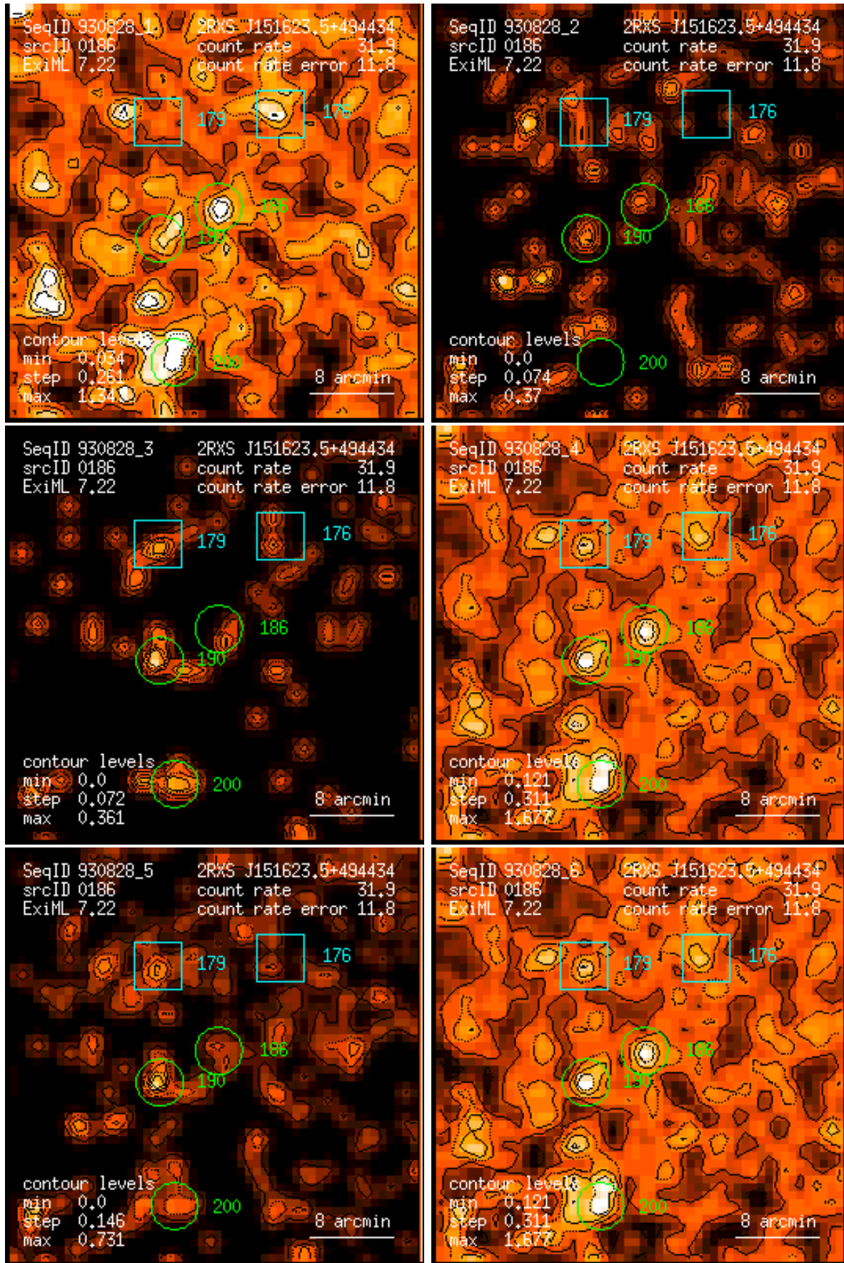
Figure 186: RASS 930828: detection 0186: band rate images, Gaussian filter: (1) PSPC channels 11 – 41, (2) 52 – 90, (3) 91 – 201, (4) 11 – 235, (5) 52 – 201, (6) 11 – 201. Broad band rates in counts/ks. Band rate contour levels in counts/ks/arcmin 2 .
