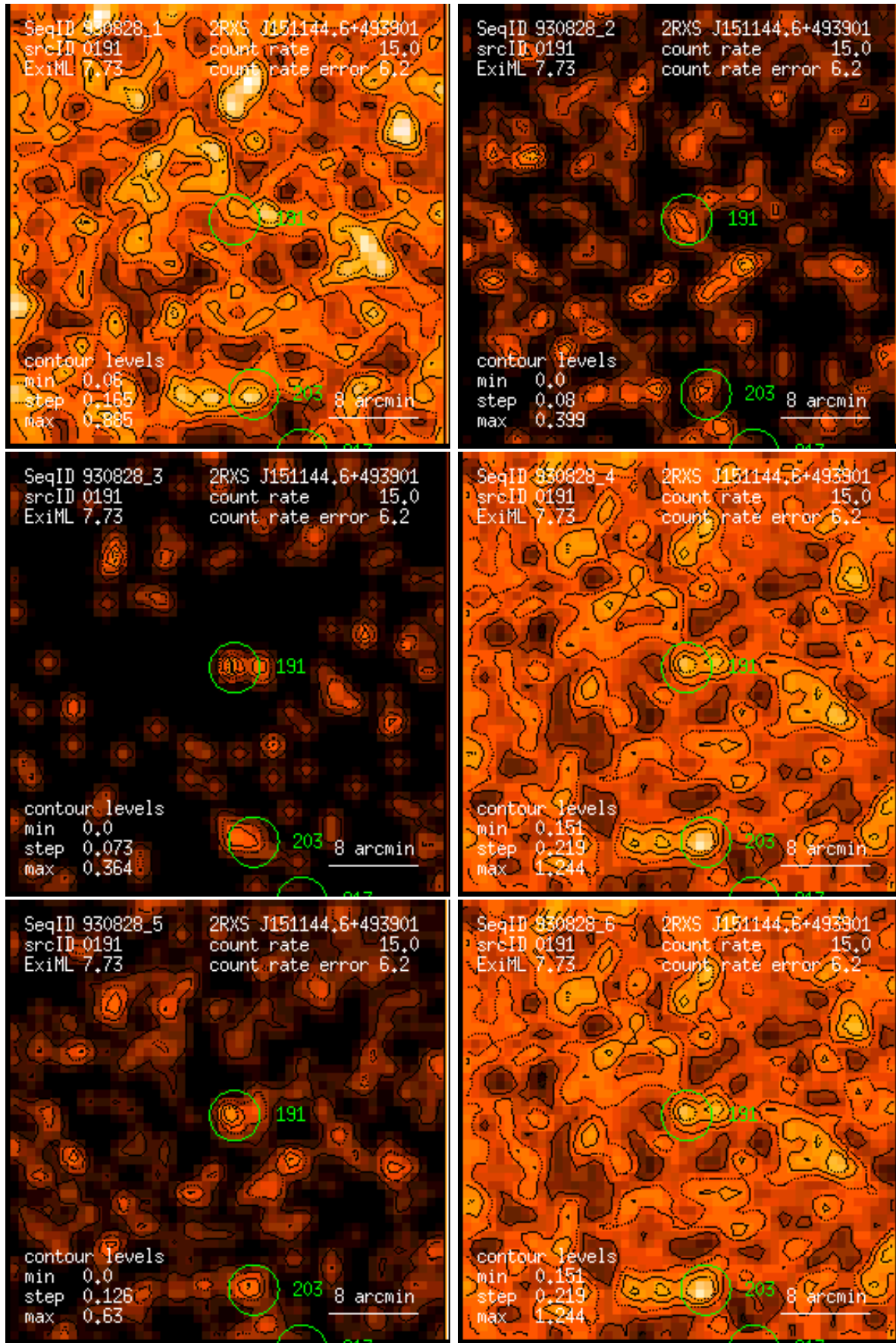
Figure 191: RASS 930828: detection 0191: band rate images, Gaussian filter: (1) PSPC channels 11 – 41, (2) 52 – 90, (3) 91 – 201, (4) 11 – 235, (5) 52 – 201, (6) 11 – 201. Broad band rates in counts/ks. Band rate contour levels in counts/ks/arcmin 2 .
