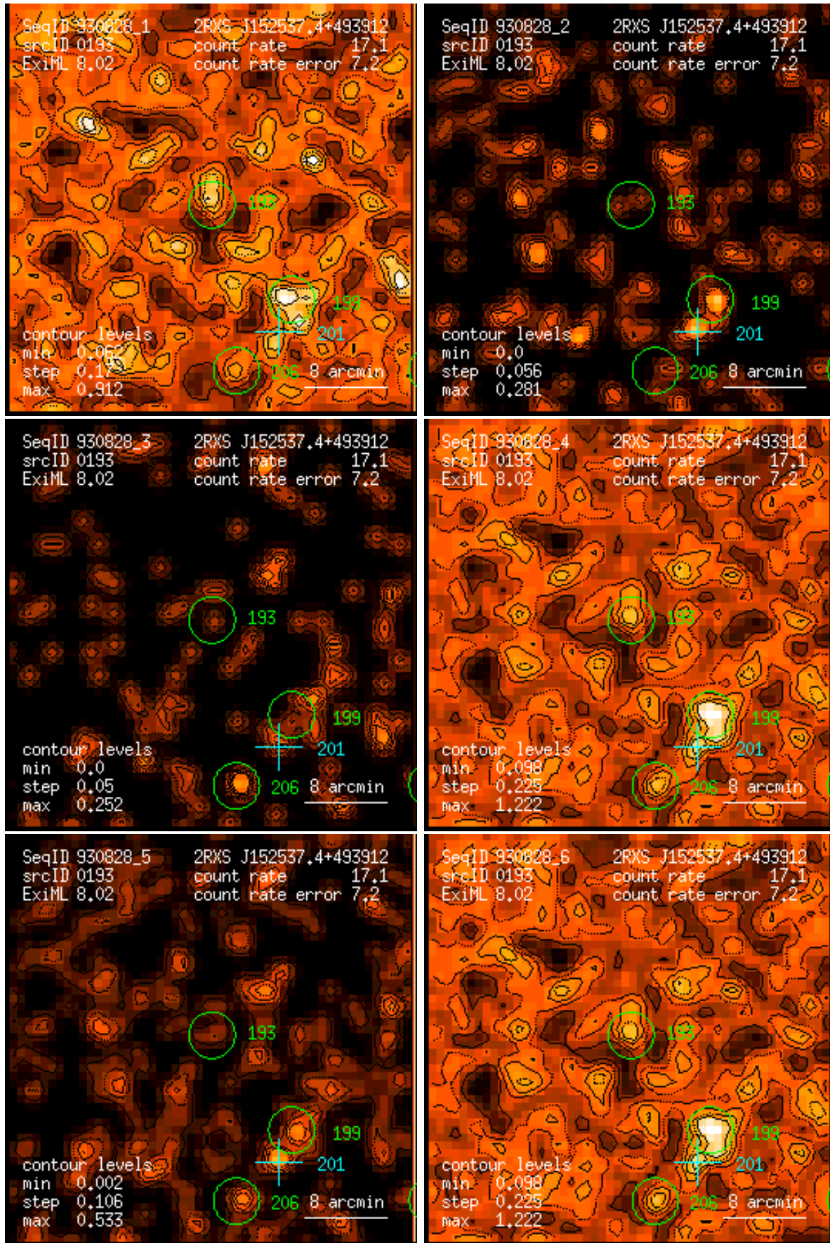
Figure 193: RASS 930828: detection 0193: band rate images, Gaussian filter: (1) PSPC channels 11 – 41, (2) 52 – 90, (3) 91 – 201, (4) 11 – 235, (5) 52 – 201, (6) 11 – 201. Broad band rates in counts/ks. Band rate contour levels in counts/ks/arcmin 2 .
