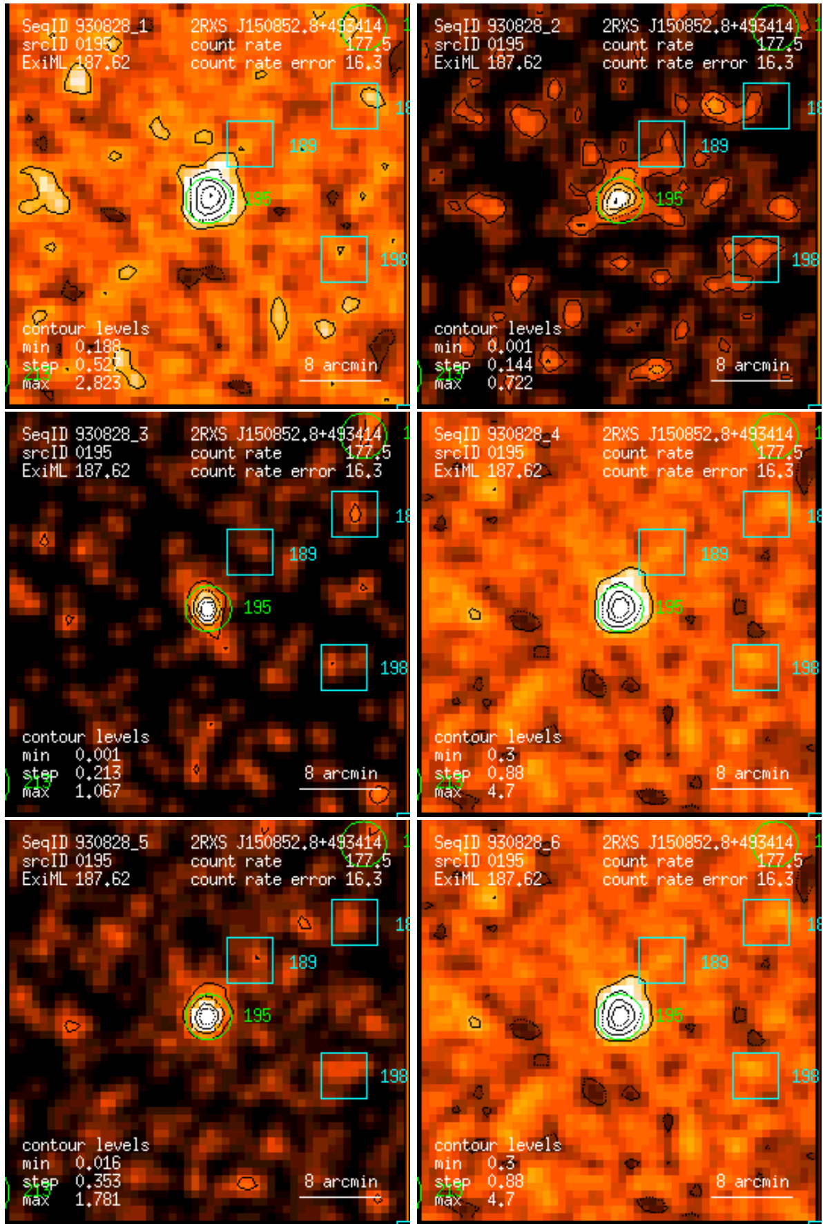
Figure 195: RASS 930828: detection 0195: band rate images, Gaussian filter: (1) PSPC channels 11 – 41, (2) 52 – 90, (3) 91 – 201, (4) 11 – 235, (5) 52 – 201, (6) 11 – 201. Broad band rates in counts/ks. Band rate contour levels in counts/ks/arcmin 2 .
