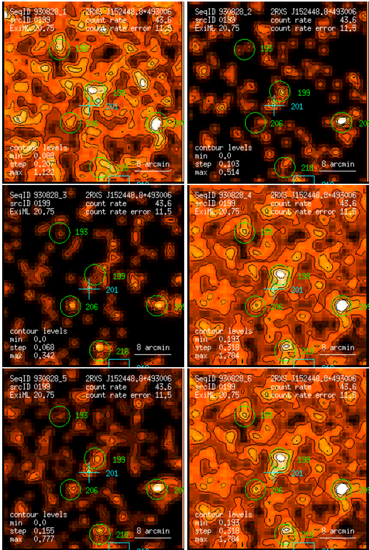
Figure 199: RASS 930828: detection 0199: band rate images, Gaussian filter: (1) PSPC channels 11 – 41, (2) 52 – 90, (3) 91 – 201, (4) 11 – 235, (5) 52 – 201, (6) 11 – 201. Broad band rates in counts/ks. Band rate contour levels in counts/ks/arcmin 2 .
