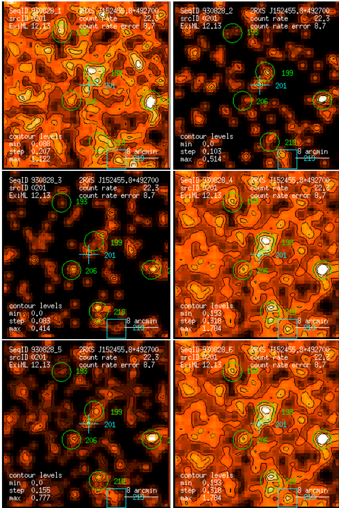
Figure 201: RASS 930828: detection 0201: band rate images, Gaussian filter: (1) PSPC channels 11 – 41, (2) 52 – 90, (3) 91 – 201, (4) 11 – 235, (5) 52 – 201, (6) 11 – 201. Broad band rates in counts/ks. Band rate contour levels in counts/ks/arcmin 2 .
