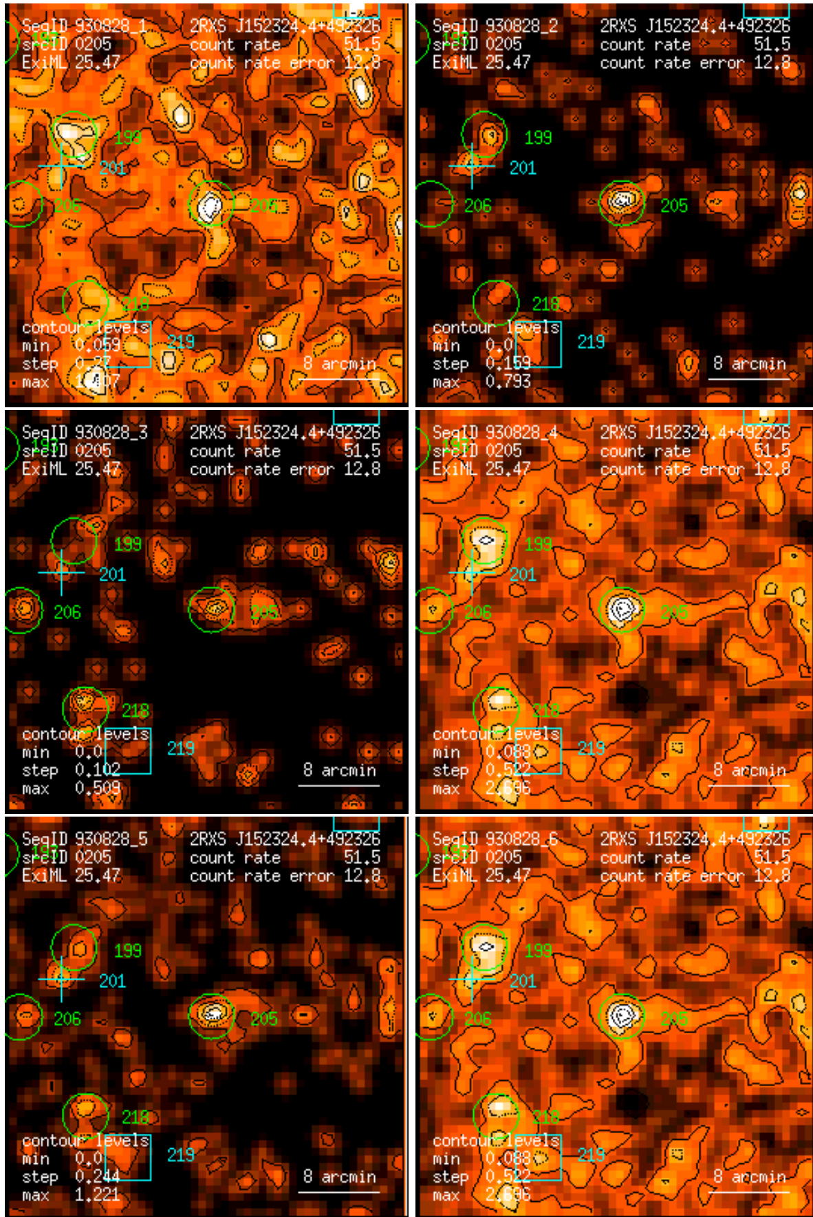
Figure 205: RASS 930828: detection 0205: band rate images, Gaussian filter: (1) PSPC channels 11 – 41, (2) 52 – 90, (3) 91 – 201, (4) 11 – 235, (5) 52 – 201, (6) 11 – 201. Broad band rates in counts/ks. Band rate contour levels in counts/ks/arcmin 2 .
