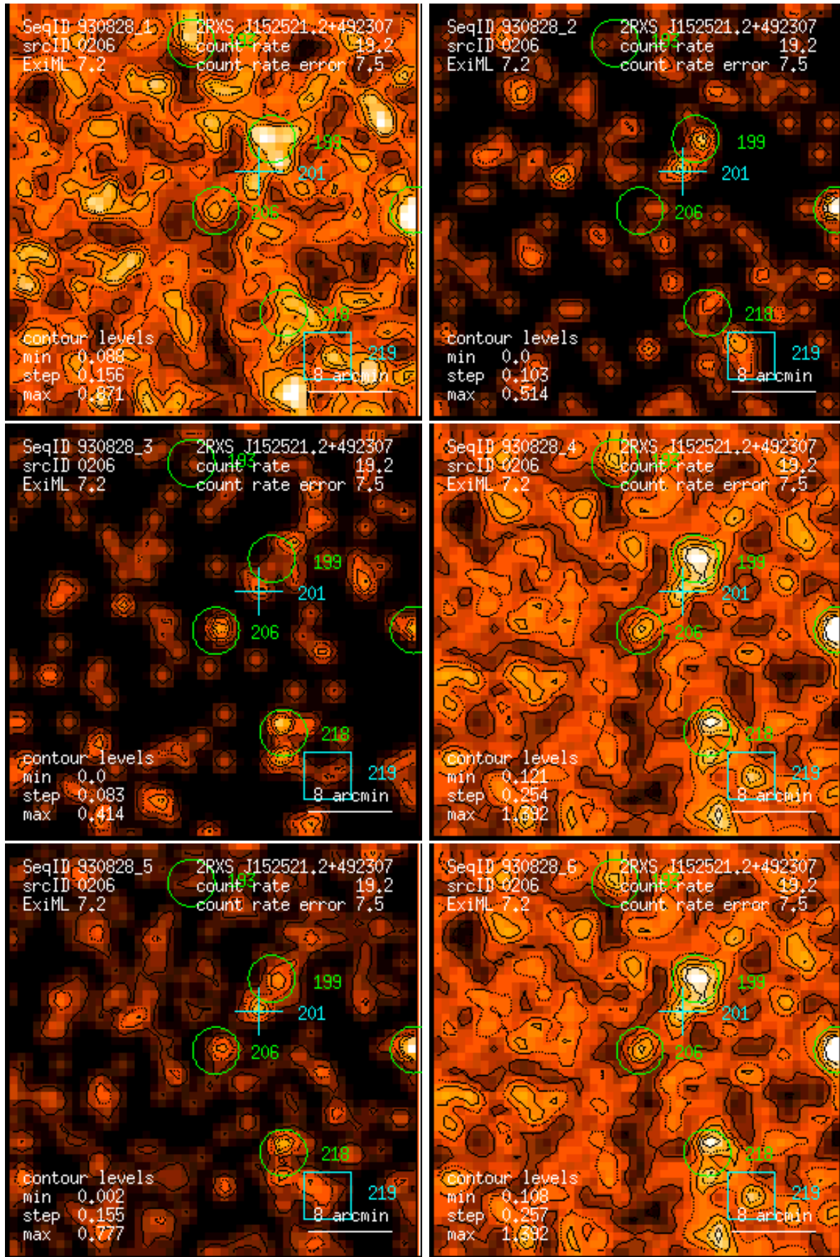
Figure 206: RASS 930828: detection 0206: band rate images, Gaussian filter: (1) PSPC channels 11 – 41, (2) 52 – 90, (3) 91 – 201, (4) 11 – 235, (5) 52 – 201, (6) 11 – 201. Broad band rates in counts/ks. Band rate contour levels in counts/ks/arcmin 2 .
