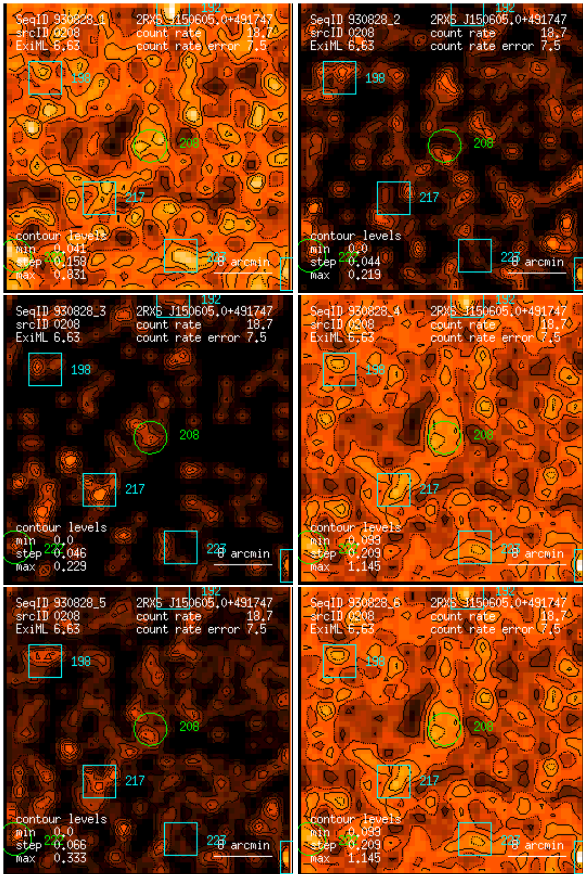
Figure 208: RASS 930828: detection 0208: band rate images, Gaussian filter: (1) PSPC channels 11 – 41, (2) 52 – 90, (3) 91 – 201, (4) 11 – 235, (5) 52 – 201, (6) 11 – 201. Broad band rates in counts/ks. Band rate contour levels in counts/ks/arcmin 2 .
