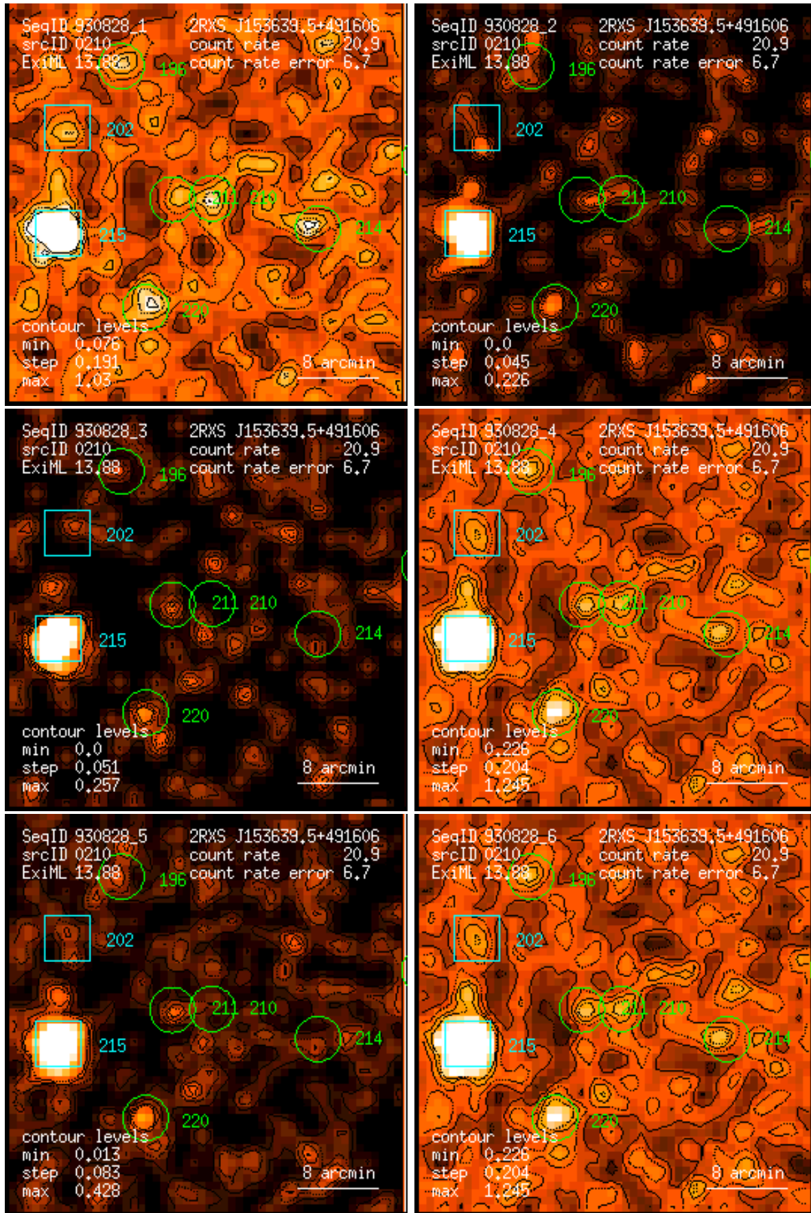
Figure 210: RASS 930828: detection 0210: band rate images, Gaussian filter: (1) PSPC channels 11 – 41, (2) 52 – 90, (3) 91 – 201, (4) 11 – 235, (5) 52 – 201, (6) 11 – 201. Broad band rates in counts/ks. Band rate contour levels in counts/ks/arcmin 2 .
