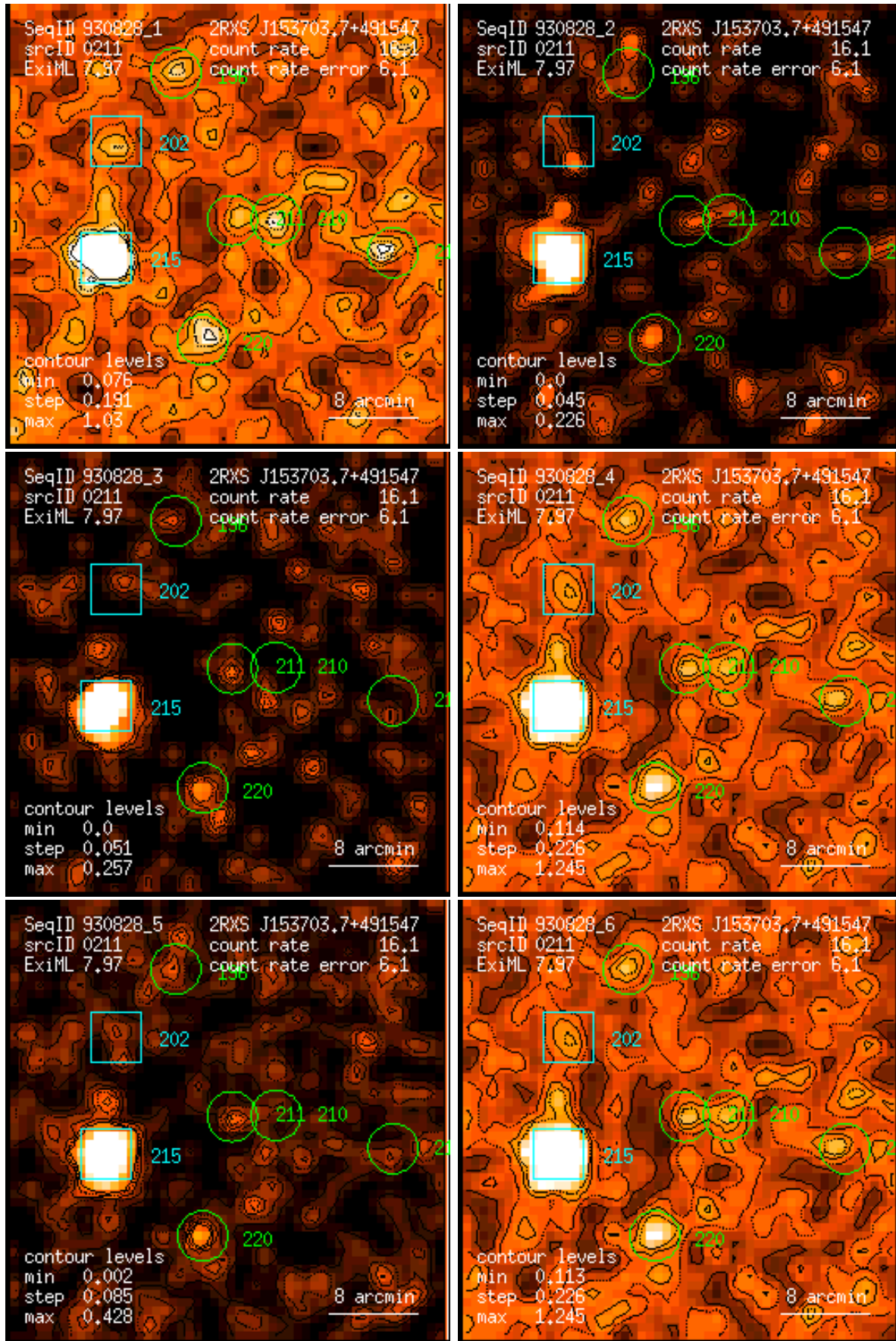
Figure 211: RASS 930828: detection 0211: band rate images, Gaussian filter: (1) PSPC channels 11 – 41, (2) 52 – 90, (3) 91 – 201, (4) 11 – 235, (5) 52 – 201, (6) 11 – 201. Broad band rates in counts/ks. Band rate contour levels in counts/ks/arcmin 2 .
