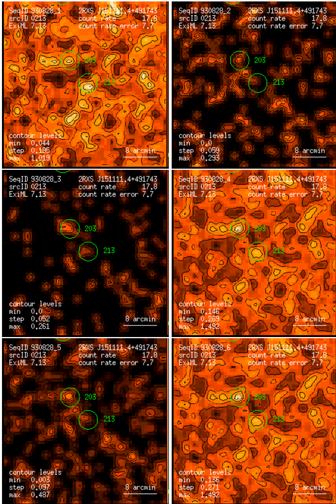
Figure 213: RASS 930828: detection 0213: band rate images, Gaussian filter: (1) PSPC channels 11 – 41, (2) 52 – 90, (3) 91 – 201, (4) 11 – 235, (5) 52 – 201, (6) 11 – 201. Broad band rates in counts/ks. Band rate contour levels in counts/ks/arcmin 2 .
