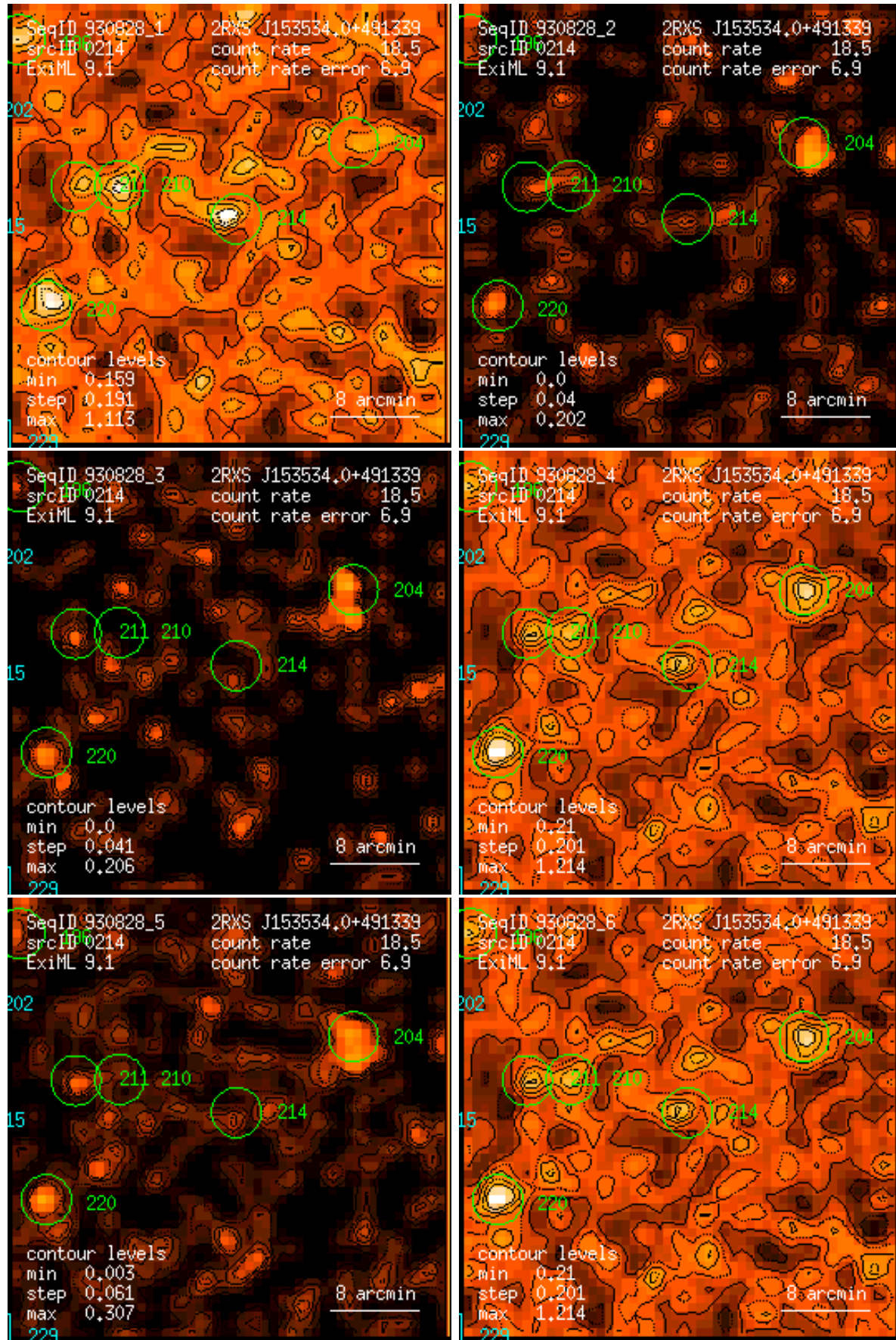
Figure 214: RASS 930828: detection 0214: band rate images, Gaussian filter: (1) PSPC channels 11 – 41, (2) 52 – 90, (3) 91 – 201, (4) 11 – 235, (5) 52 – 201, (6) 11 – 201. Broad band rates in counts/ks. Band rate contour levels in counts/ks/arcmin 2 .
