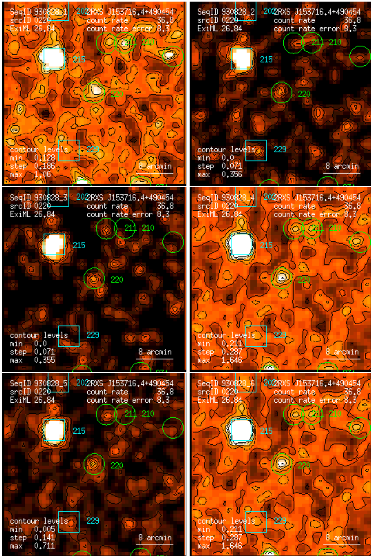
Figure 220: RASS 930828: detection 0220: band rate images, Gaussian filter: (1) PSPC channels 11 – 41, (2) 52 – 90, (3) 91 – 201, (4) 11 – 235, (5) 52 – 201, (6) 11 – 201. Broad band rates in counts/ks. Band rate contour levels in counts/ks/arcmin 2 .
