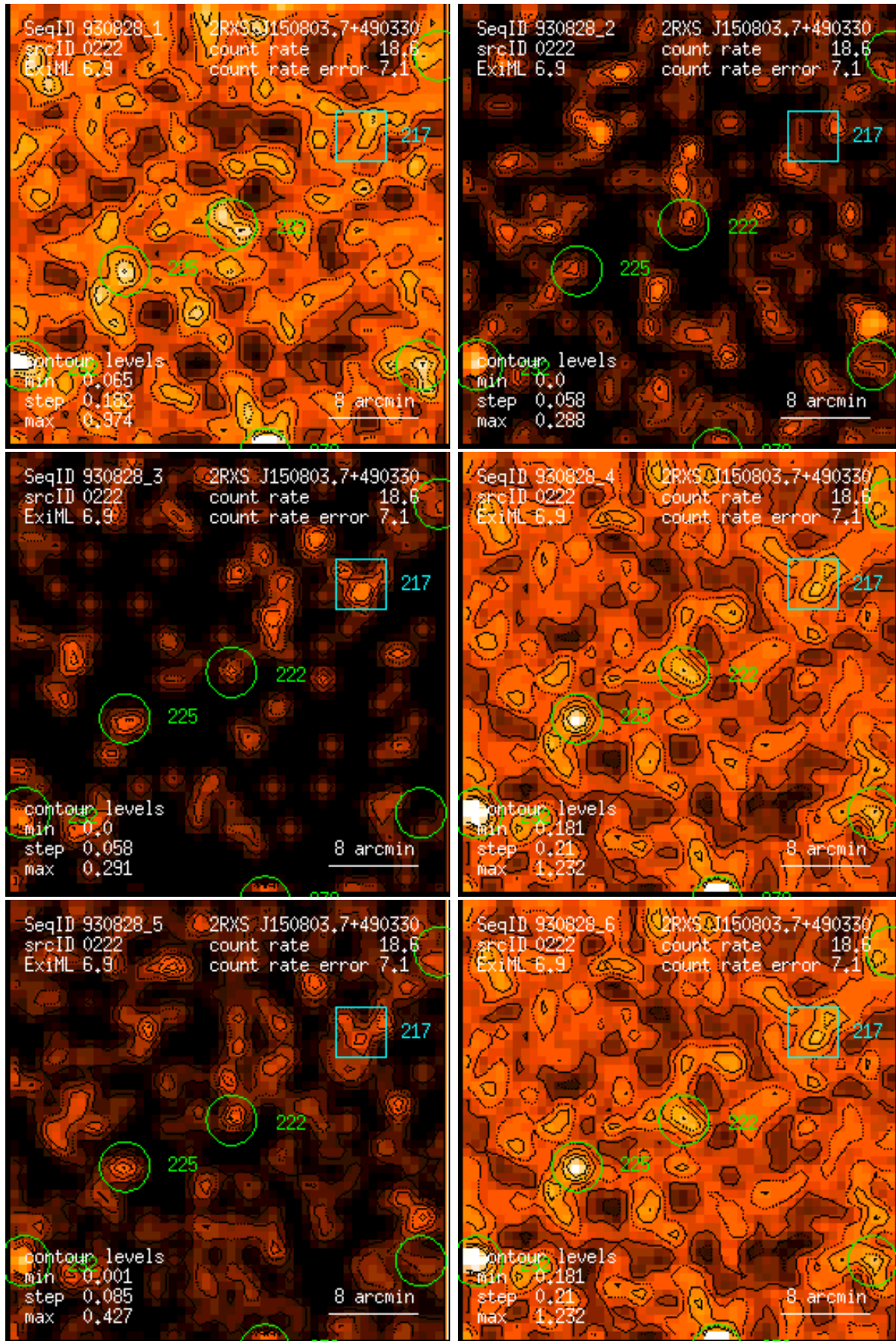
Figure 222: RASS 930828: detection 0222: band rate images, Gaussian filter: (1) PSPC channels 11 – 41, (2) 52 – 90, (3) 91 – 201, (4) 11 – 235, (5) 52 – 201, (6) 11 – 201. Broad band rates in counts/ks. Band rate contour levels in counts/ks/arcmin 2 .
