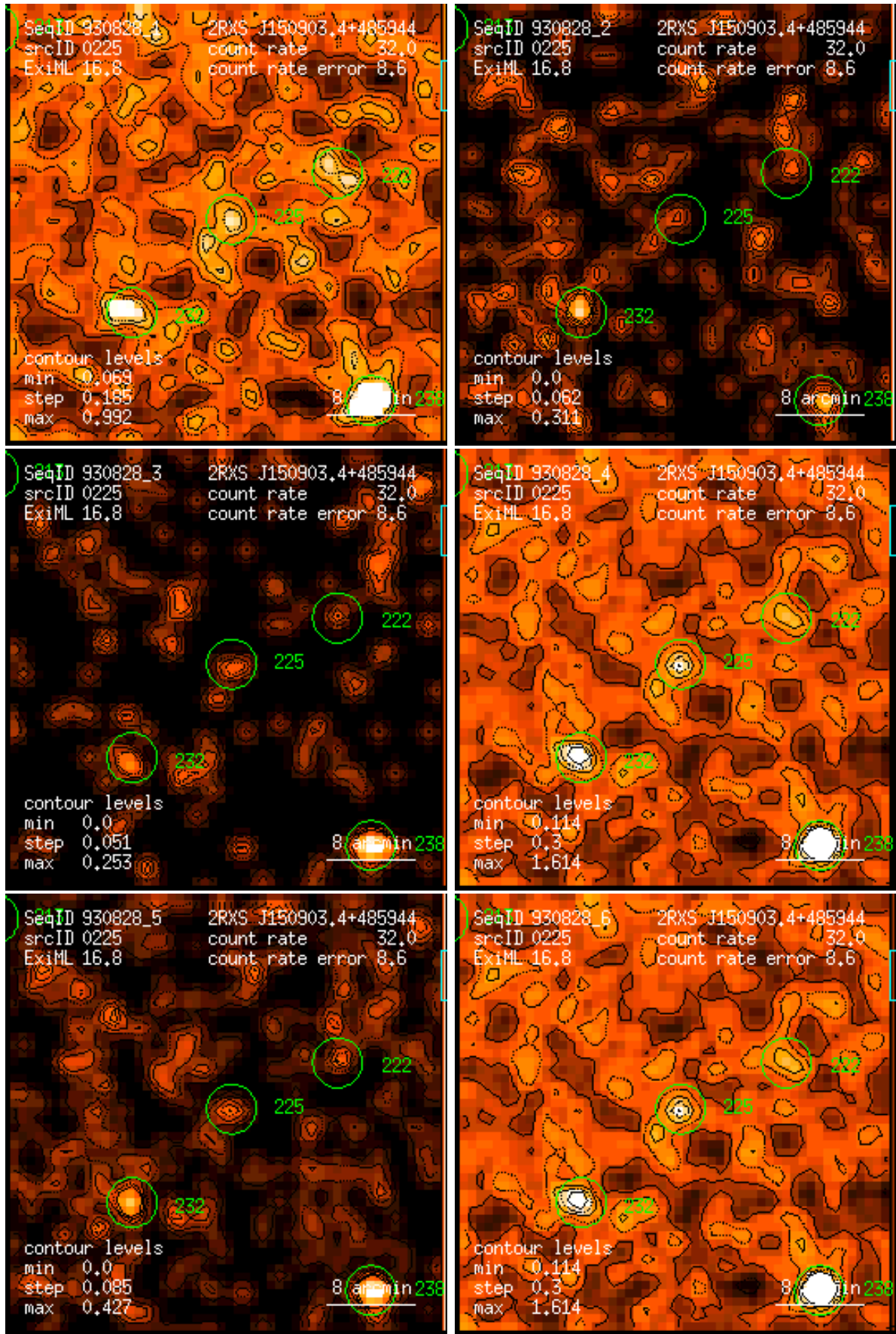
Figure 225: RASS 930828: detection 0225: band rate images, Gaussian filter: (1) PSPC channels 11 – 41, (2) 52 – 90, (3) 91 – 201, (4) 11 – 235, (5) 52 – 201, (6) 11 – 201. Broad band rates in counts/ks. Band rate contour levels in counts/ks/arcmin 2 .
