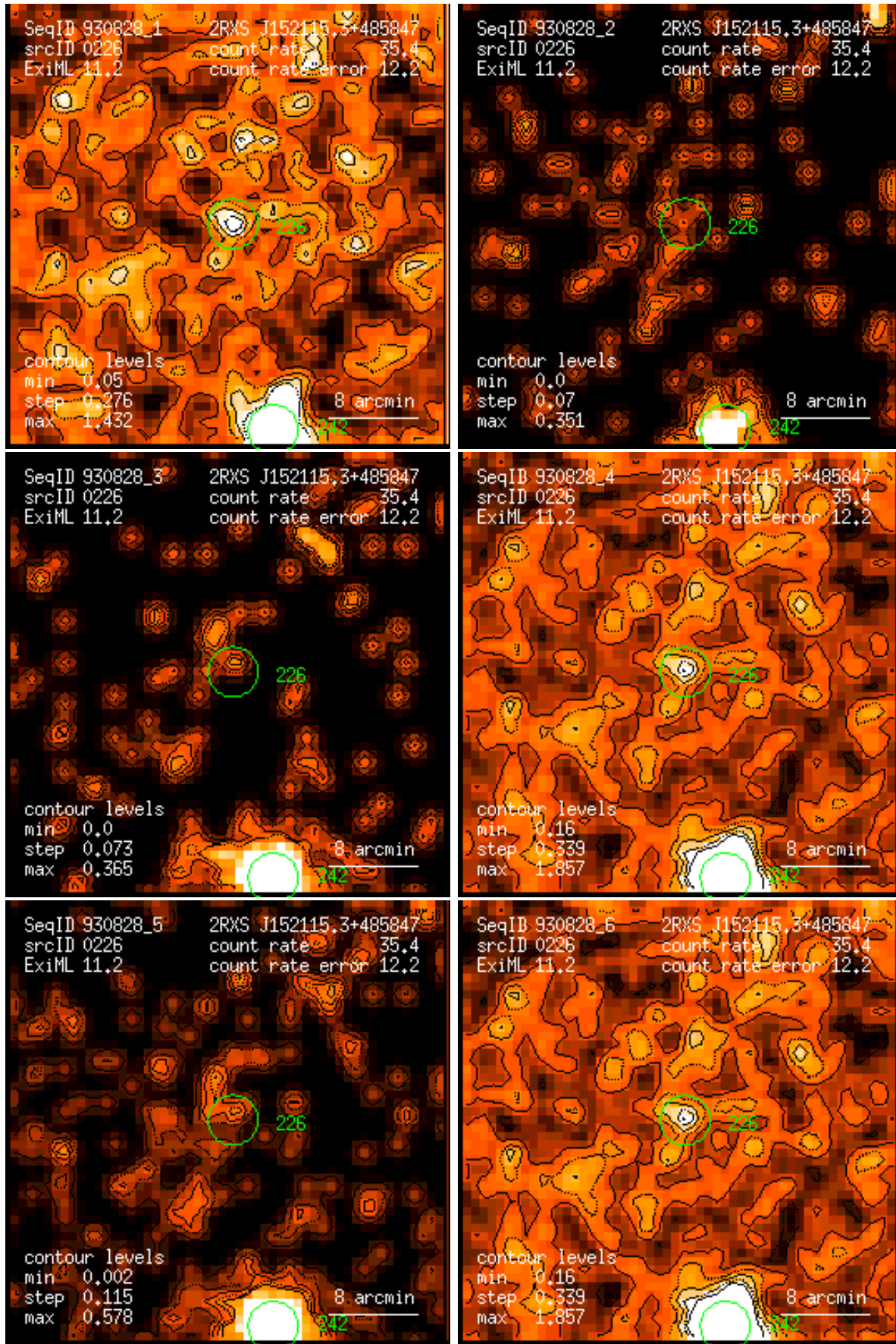
Figure 226: RASS 930828: detection 0226: band rate images, Gaussian filter: (1) PSPC channels 11 – 41, (2) 52 – 90, (3) 91 – 201, (4) 11 – 235, (5) 52 – 201, (6) 11 – 201. Broad band rates in counts/ks. Band rate contour levels in counts/ks/arcmin 2 .
