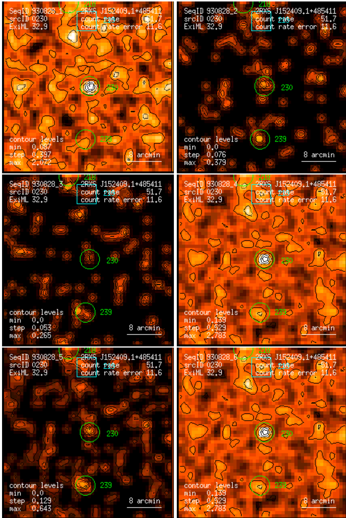
Figure 230: RASS 930828: detection 0230: band rate images, Gaussian filter: (1) PSPC channels 11 – 41, (2) 52 – 90, (3) 91 – 201, (4) 11 – 235, (5) 52 – 201, (6) 11 – 201. Broad band rates in counts/ks. Band rate contour levels in counts/ks/arcmin 2 .
