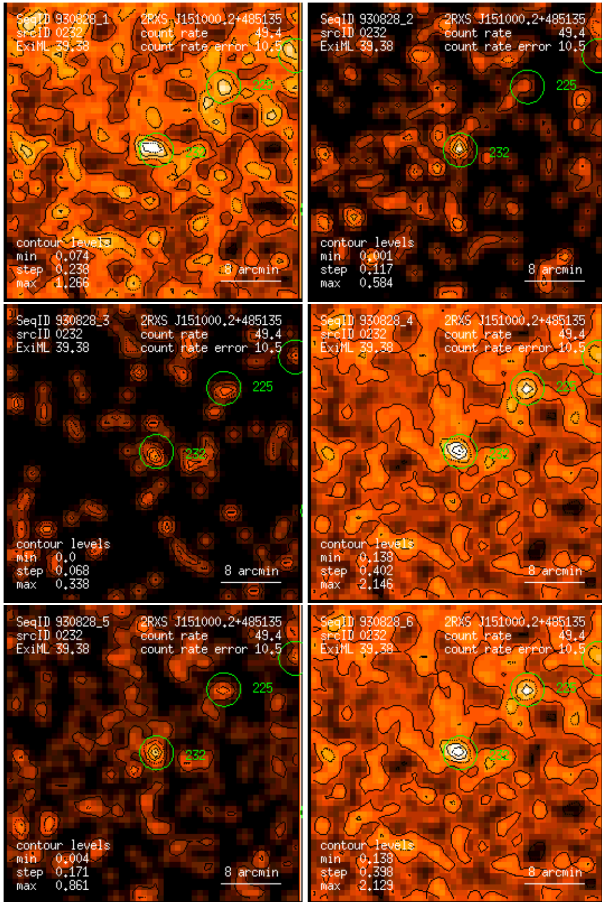
Figure 232: RASS 930828: detection 0232: band rate images, Gaussian filter: (1) PSPC channels 11 – 41, (2) 52 – 90, (3) 91 – 201, (4) 11 – 235, (5) 52 – 201, (6) 11 – 201. Broad band rates in counts/ks. Band rate contour levels in counts/ks/arcmin 2 .
